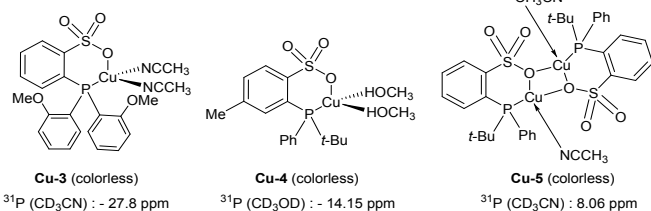
Scheme 2. Impact of the chelate and solvent on nuclearity.
