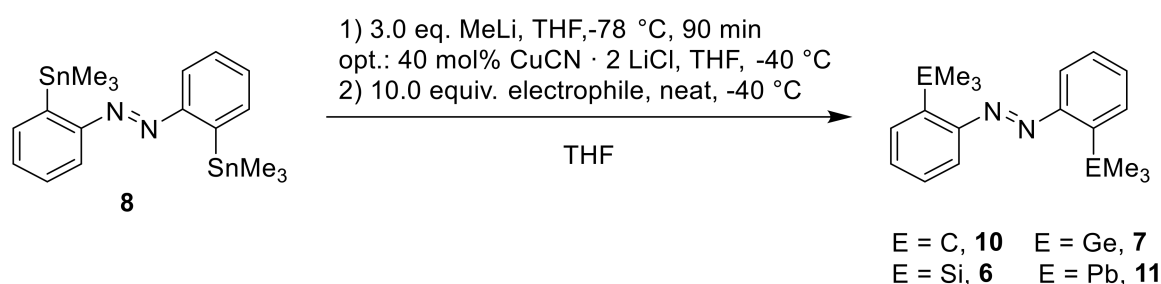
Scheme 8. Metalation to obtain di-methylated azobenzenes 10 , 11 and 6 , 7 .
