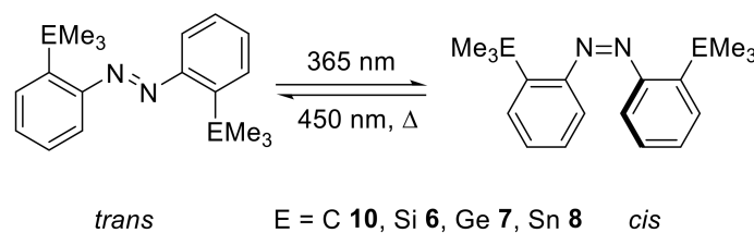
Scheme 10. Light/thermally induced isomerization of synthesized azobenzenes 10 and 6–8 .
