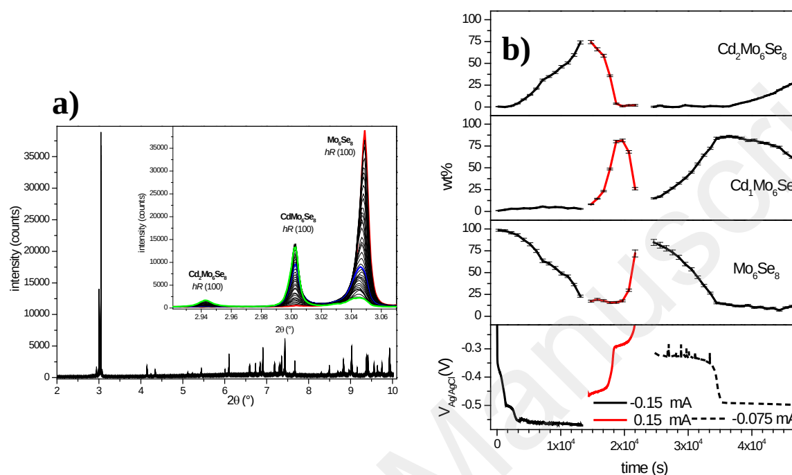
Figure 2: part a) In situ diffraction pattern during galvanostatic intercalation in \text{Mo}_6\text{Se}_8 : part a) typical pattern (inset: zoom around the reflection of the different phases during the first intercalation stage); part b) from top to bottom: estimated phase fractions and corresponding voltage evolution as a function of time.
