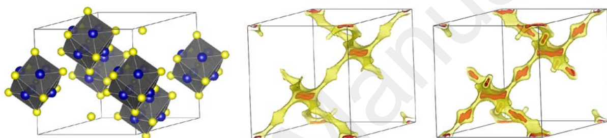
Figure 10: Part a) Chevrel phases in hexagonal setting ( R\bar{3}:hP ), BVSE map for \text{Cd}_1\text{Mo}_6\text{Se}_8 and \text{Cd}_2\text{Mo}_6\text{Se}_8 part b) and c), respectively. Red and yellow isosurfaces corresponds to 0.3 and 0.5 eV above the minimum and the percolation energy, respectively.
