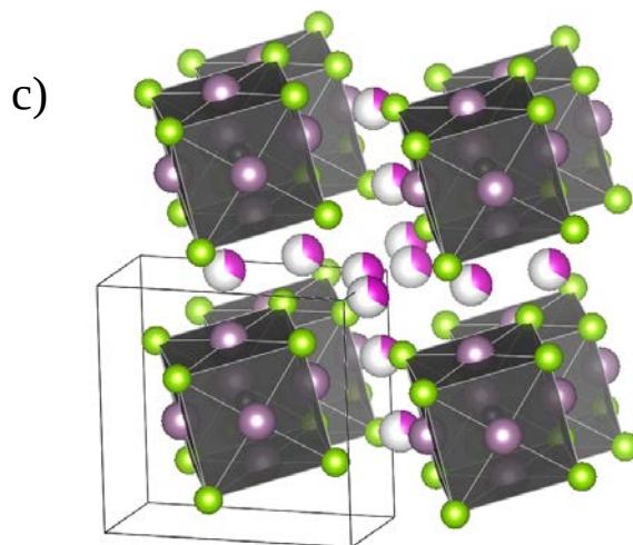
Figure 9: \text{Cd}_2\text{Mo}_6\text{Se}_8 . Part a) MEM electronic density map within the a - b plane at z=0.4444 ( hP ) showing three maxima corresponding to the three in-plane Cd2 atoms, shifted from the ideal 9d Wyckoff site at \frac{1}{2} 0 \frac{1}{2} (max./min. saturation levels at 10/0 \text{ e}^-/\text{\AA}^{-3} ). Part b) MEM electronic density map within the a - b plane centered at \frac{2}{3} \frac{1}{3} 0.3194 cavity 1, same zoom, orientation and scale of Figure 8 a). Part c) Graphical representation of the \text{Cd}_2\text{Mo}_6\text{Se}_8 structure in the hR setting.
