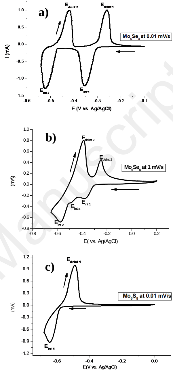
Figure 1 : cyclic voltammetry of part a) and b) \text{Mo}_6\text{Se}_8 at two different cycling rate part c) of \text{Mo}_6\text{S}_8 with the rate 0.01 mV/s for 0.1 M solutions of \text{Cd}^{2+} ;
