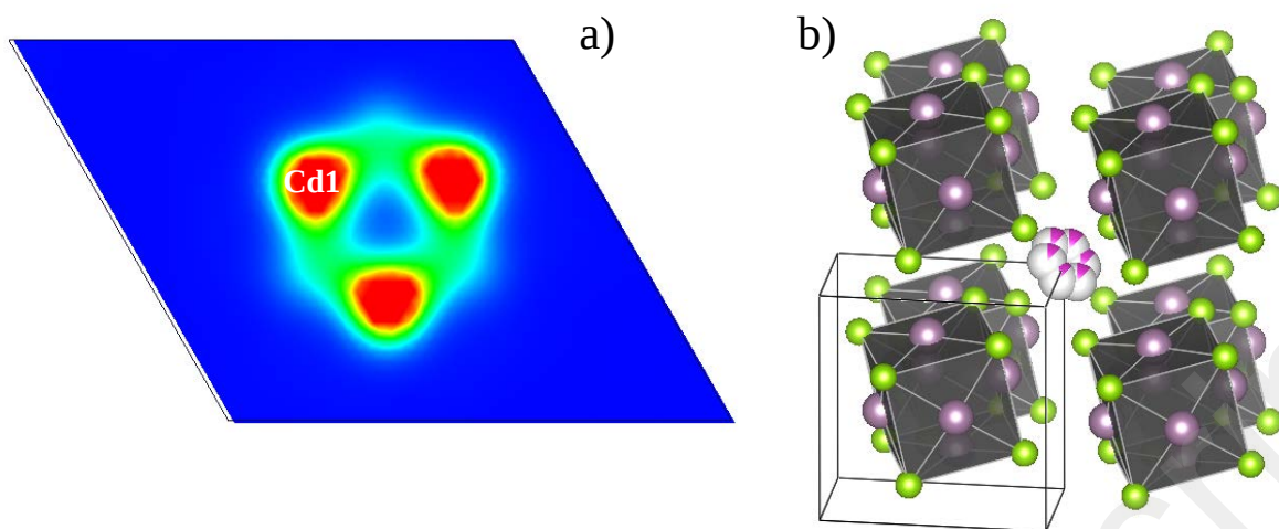
Figure 8: \text{Cd}_1\text{Mo}_6\text{Se}_8 Part a) phase, cavity 1: MEM electronic density map within the a - b plane centered at 2/3 \ 1/3 \ 0.3194 showing three maxima corresponding to the three in-plane Cd1 atoms (max./min. saturation levels at 30/0 \text{ e}^-/\text{\AA}^{-3} ). Part b) graphical representation of the \text{Cd}_1\text{Mo}_6\text{Se}_8 structure in the rhombohedral cell.
