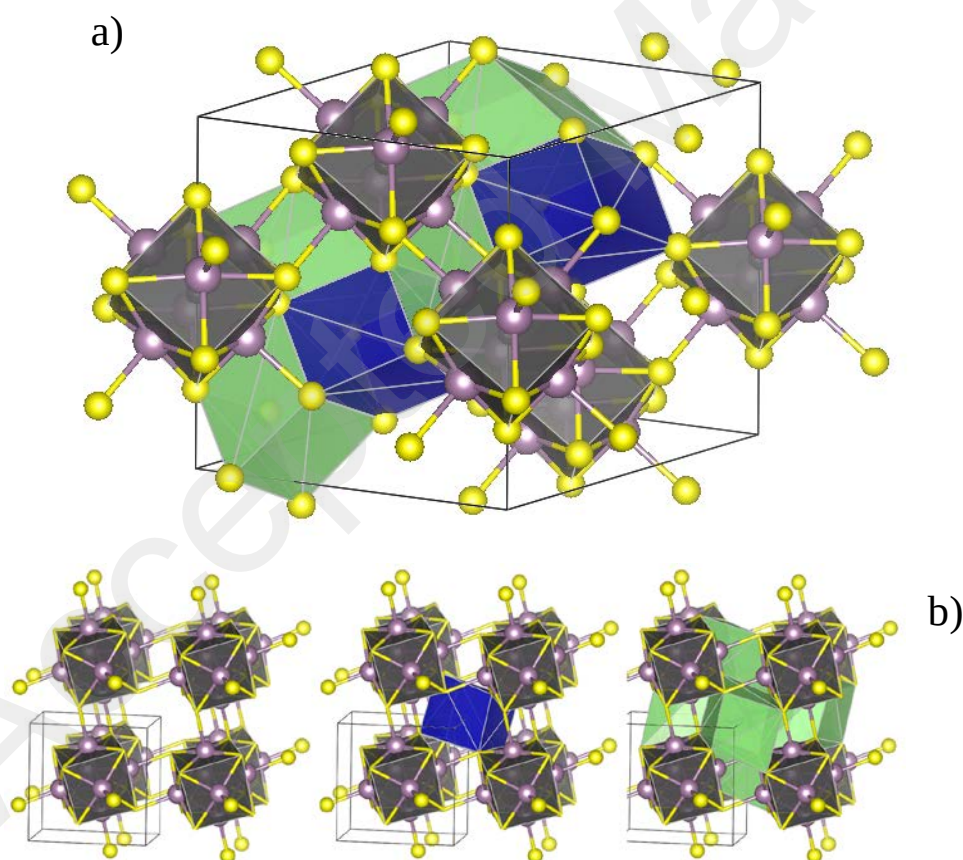
Figure 5: Part a) General structural model for Chevrel phases in hexagonal setting ( R\bar{3}:hP ) with cavity 1 and 2, blue and green polyhedra. Part b) \text{Mo}_6\text{X}_8 blocks simple cubic packing in
