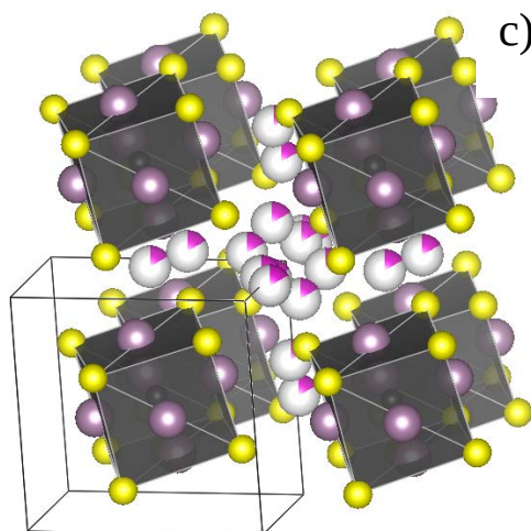
Figure 7: \text{Cd}_2\text{Mo}_6\text{S}_8 . Part a) Cavity 2: MEM electronic density map within the a - b plane at z=0.5347 showing three maxima corresponding to the three in-plane Cd2 atoms, shifted from the ideal 9d Wyckoff site at \frac{1}{2} 0 \frac{1}{2} (max./min. saturation levels at 8/0 \text{ e}^-/\text{\AA}^{-3} ). Part b) Cavity 1: MEM electronic density map within the a - b plane focused on cavity 1, z=0.3472 ( hP setting). Max./min. saturation levels at 5/0 \text{ e}^- \cdot \text{\AA}^{-3} . Part b) Graphical representation of the \text{Cd}_2\text{Mo}_6\text{S}_8 structure in the rhombohedral cell.
