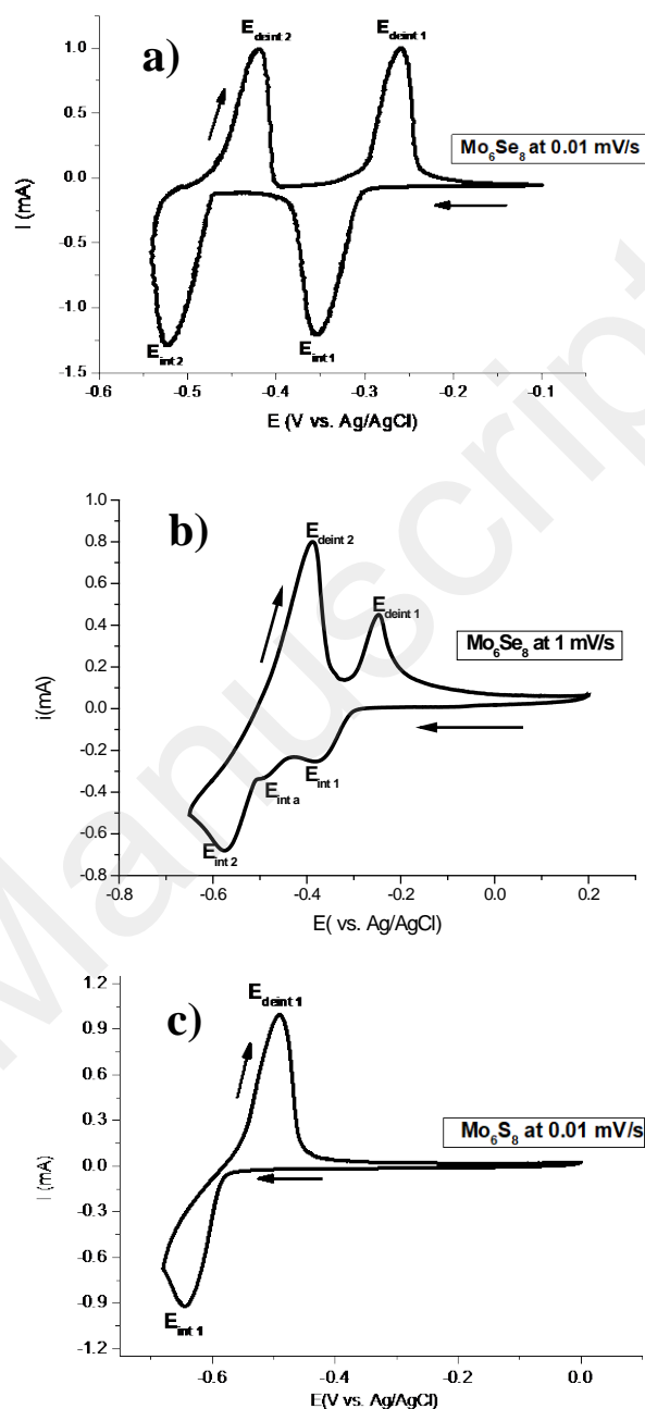
Figure 1 : cyclic voltammetry of part a) and b) Mo_6Se_8 at two different cycling rate part c) of Mo_6S_8 with the rate 0.01 mV/s for 0.1 M solutions of Cd^{2+} ;
