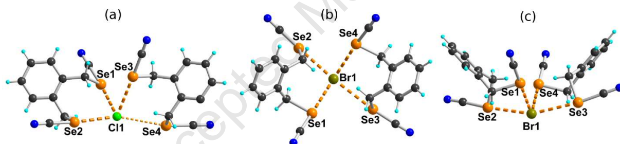
Figure 4. Detail of: (a) the \text{Cl}^- and (b,c) the \text{Br}^- environment in the crystal structures of (a): (\mathbf{1})_2 \cdot \text{PPh}_4\text{Cl} \cdot \text{Et}_2\text{O} and (b,c): (\mathbf{1})_2 \cdot \text{PPh}_4\text{Br} (orthorhombic phase).
