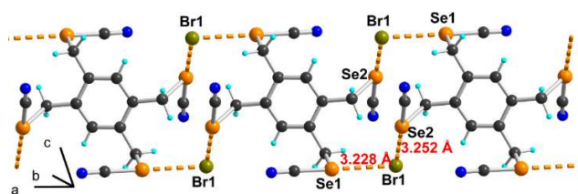
Figure 3. Detail of the ChB chains running along a in 2\bullet(\text{PPh}_4\text{Br})_2 .
