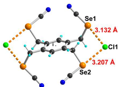
Figure 2. Detail of the interaction between 2 and \text{Cl}^- in 2\bullet(\text{PPh}_4\text{Cl})_2
