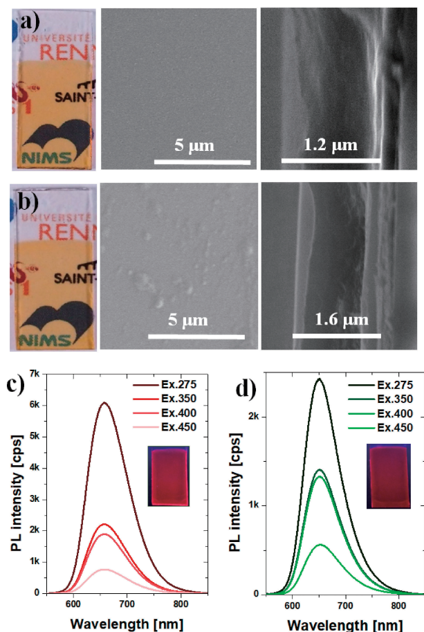
Figure 8. Photographs (size of ITO glass is 1 \times 2 cm), surface morphology and cross section SEM images of deposited films: a) 4@CAP and b) 4@PMMA. The photoluminescence of the c) 4@CAP and d) 4@PMMA films.
