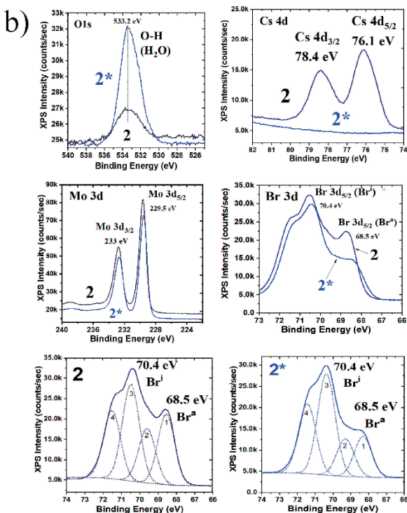
Figure 5. (a) The EDX-HRTEM mapping of Cs, Mo and Br elements of the \text{Mo}_6 based thin film. (b) XPS spectrum of powder (2) and thin film (2*) based on cluster 2.
