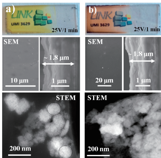
Figure 13. Photographs (size of ITO glass is 1 \times 2 cm) (upper); HR-SEM images of surface morphologies and cross sections (middle); STEM images (lower) of the Nb 6 -based cluster anodic films: a) 6@PMMA, and b) 7@PMMA.
