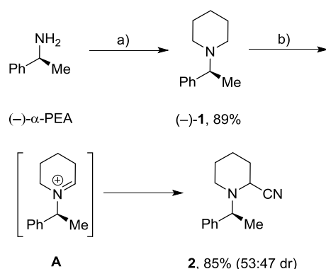
Scheme 2. Anodic cyanation of piperidine (-)- 1 . Reagents and conditions: (a) (S)-(-)- \alpha -PEA, 1,5-dibromopentane, K_2CO_3 , DMSO, 50 °C, 2 h, then 100 °C, 2 h. (b) MeOH/ LiClO_4 \cdot 3H_2O , NaCN, E_p = 1.0 V (ECS).
