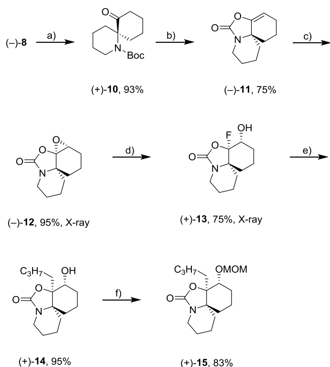
Scheme 4. Synthesis of oxazolidinone (+)- 15 . Reagents and conditions (a) \text{Boc}_2\text{O} , DIPEA, acetonitrile, reflux, 3 h. (b) TMEDA, \text{Ph}_3\text{PCl}_2 , acetonitrile, rt, 4 h. (c) Oxone, \text{Na}_2\text{B}_4\text{O}_7 \cdot 10\text{H}_2\text{O} , acetone, \text{CH}_2\text{Cl}_2 , 0 °C, 4 h. (d) \text{BF}_3 \cdot \text{Et}_2\text{O} , \text{Et}_2\text{O} , 0 °C, 1 h. (e) n\text{BuMgBr} , \text{CuCl}_2 (5 mol%), THF, rt, 2 h. (f) NaH, MOMCl, NaI (10 mol%), THF, rt, 16 h.
