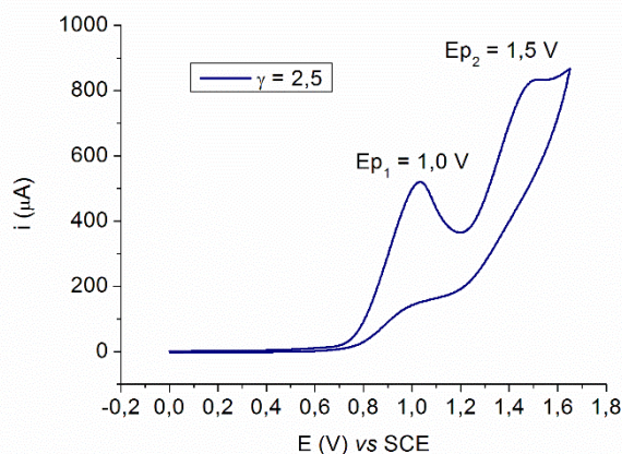
Figure 2. Cyclic Voltammogram of piperidine (-)- 1 (15 mmol). MeOH/ LiClO_4 \cdot 3H_2O (0.1 M), glassy carbon electrode, \nu = 0.05 \text{ Vs}^{-1} , NaCN (35 mmol).
