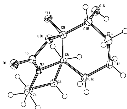
Figure 5. ORTEP view of syn -fluorohydrin (+)- 13 . Thermal ellipsoid plots are drawn at 40% probability.
