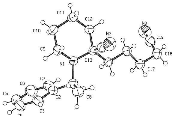
Figure 3. ORTEP view of derivative (+)-4. Thermal ellipsoid plots are drawn at 40% probability.
