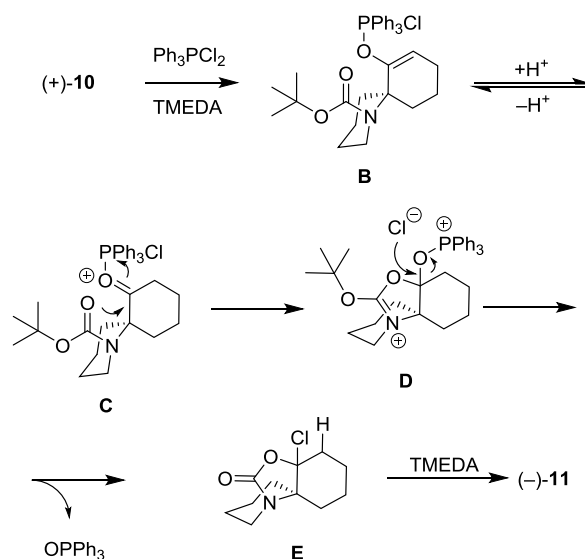
Scheme 5. Proposed mechanism for the cyclization of (+)- 10 .
