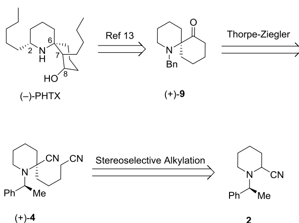
Scheme 1. Retrosynthetic analysis of (–)-PHTX from \alpha -aminonitrile 2.
