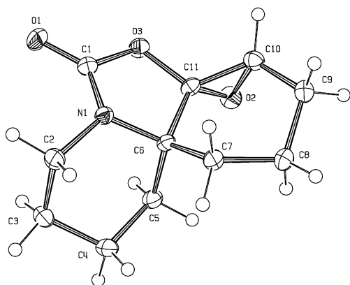
Figure 4. ORTEP view of epoxide (–)- 12 . Thermal ellipsoid plots are drawn at 40% probability.
