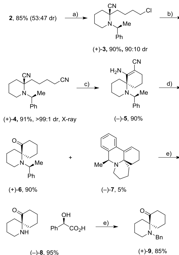
Scheme 3. Formal synthesis of (–)-HTX. reagents and conditions: (a) LDA, THF, -80\text{ }^{\circ}\text{C} to 0\text{ }^{\circ}\text{C} , 2 h, then 1-bromo-4-chlorobutane, -80\text{ }^{\circ}\text{C} to rt. (b) NaCN, \text{Bu}_4\text{NI} (10% mol), DMSO, 72 h, rt. (c) LDA, THF, -80\text{ }^{\circ}\text{C} to 0\text{ }^{\circ}\text{C} , 12 h. (d) Toluene, HCl 35%, reflux, 15 h. (e) 10% Pd/C, MeOH, \text{H}_2 (1 bar), 20\text{ }^{\circ}\text{C} , 24 h. (f) BnBr, DMSO, \text{Na}_2\text{CO}_3 , 72 h, 20\text{ }^{\circ}\text{C} .
