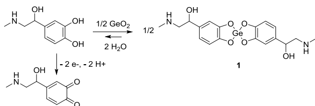
Scheme 2. Synthesis of complex 1 .
