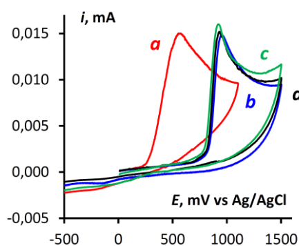
Figure 5. (a) Oxidation of 3,4-dihydroxybenzaldehyde ( 2 \text{ mmol L}^{-1} ), (b) 3,4-dihydroxybenzaldehyde-germanium bis- 2 ( 1 \text{ mmol L}^{-1} ), (c) tris-adduct 3 ( 0.67 \text{ mmol L}^{-1} ) \text{GeO}_2 ( 1 \text{ mmol L}^{-1} ), and (d) oxidation of 3,4-dihydroxybenzaldehyde ( 2 \text{ mmol L}^{-1} ) after 5 min of stay in the presence of \text{GeO}_2 ( 1 \text{ mmol L}^{-1} ). GC disk electrode ( d = 1.7 \text{ mm} ), phosphate buffer (pH = 6.86), scan rate v = 0.1 \text{ V s}^{-1} , T = 298 \text{ K} .
