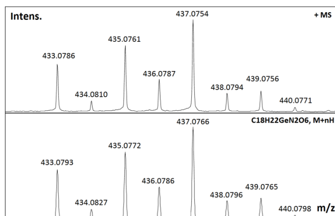
Figure 1. A fragment of the ESI-HRMS (positive ions) spectrum of 1 in H 2 O/CH 3 CN (1:1): (top) experimental, (bottom) calculated.
