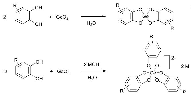
Scheme 1. Bevallard's reaction.
