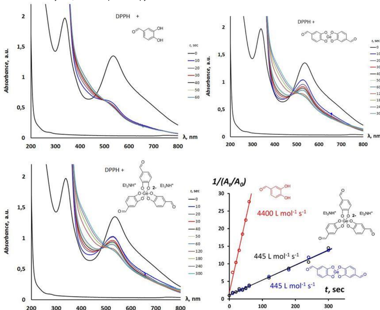
Figure 6. UV spectra of DPPH (0.1 mmol L -1 ) in phosphate buffer (pH = 6.86) in the presence of (top, left) 3,4-dihydroxybenzaldehyde (0.2 mmol L -1 ), (top, right) 3,4-dihydroxybenzaldehyde-germanium bis- (0.1 mmol L -1 ), (bottom, left) tris-adduct (0.067 mmol L -1 ) and (bottom, right) kinetic curves of interaction of compounds 2 , 3 and 3,4-dihydroxybenzaldehyde with DPPH.
