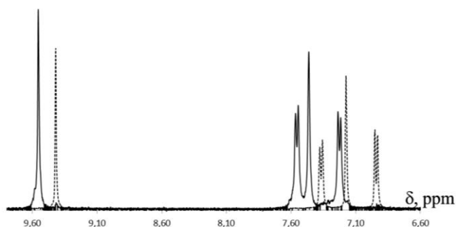
Figure 7. ^1\text{H} NMR spectra of 2 (line) and 3 (dotted line) in DMSO (300 MHz, 298 K).
