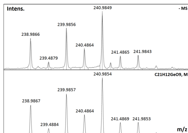
Figure 4. Fragments of the ESI-HRMS negative ion spectrum of 2 in \text{H}_2\text{O}/\text{CH}_3\text{CN} (1:1): (top) experimental, (bottom) calculated.
