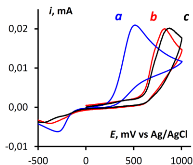
Figure 2. (a) Oxidation of adrenaline (2 mmol L -1 ), (b) adrenaline-germanium complex 1 (1 mmol L -1 ), and (c) adrenaline-GeO 2 mixture (2 + 1 mmol L -1 ) at a glassy carbon (GC) disk electrode (d = 1.7 mm) in phosphate buffer (pH = 6.86). Scan rate v = 0.1 V s -1 . T = 298 K.
