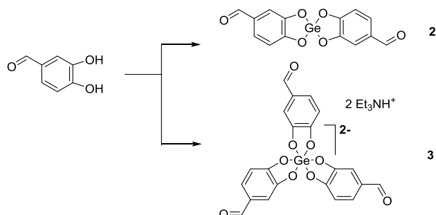
Scheme 3. Synthesis of complexes 2 and 3 .
