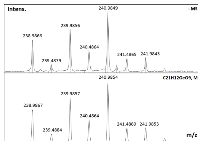
Figure 4. Fragments of the ESI-HRMS negative ion spectrum of 2 in H 2 O/CH 3 CN (1:1): (top) experimental, (bottom) calculated.
