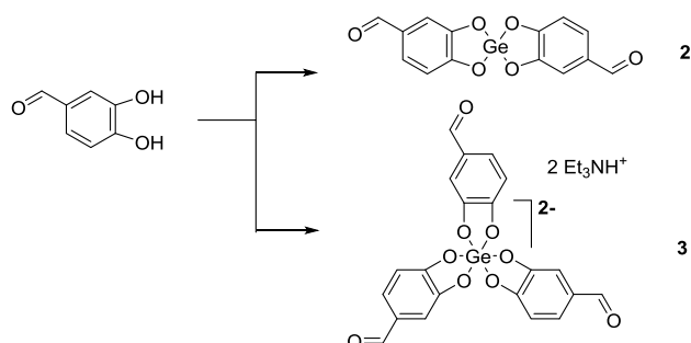
Scheme 3. Synthesis of complexes 2 and 3 .
