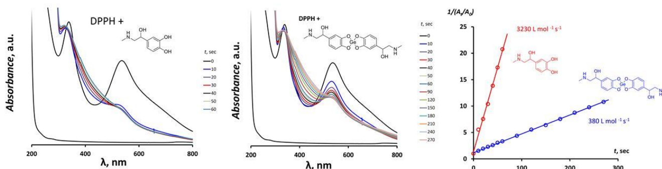
Figure 3. UV spectra of DPPH ( 0.1 \text{ mmol L}^{-1} ) in phosphate buffer ( \text{pH} = 6.86 ) in the presence of (left) adrenaline ( 0.2 \text{ mmol L}^{-1} ), (centre) adrenaline-germanium adduct ( 0.1 \text{ mmol L}^{-1} ) and kinetic curves (right) of interaction of compound 1 and adrenaline with DPPH.
