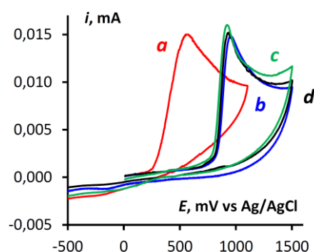
Figure 5. (a) Oxidation of 3,4-dihydroxybenzaldehyde (2 mmol L -1 ), (b) 3,4-dihydroxybenzaldehyde-germanium bis-2 (1 mmol L -1 ), (c) tris-adduct 3 (0.67 mmol L -1 ) GeO 2 (1 mmol L -1 ), and (d) oxidation of 3,4-dihydroxybenzaldehyde (2 mmol L -1 ) after 5 min of stay in the presence of GeO 2 (1 mmol L -1 ). GC disk electrode (d = 1.7 mm), phosphate buffer (pH = 6.86), scan rate v = 0.1 V s -1 , T = 298 K.
