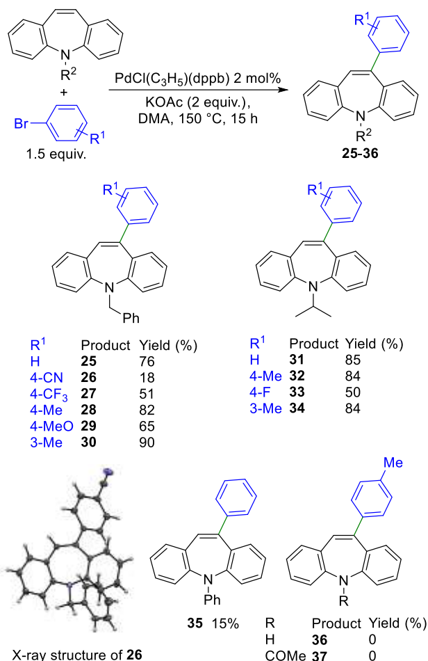
Scheme 3. Palladium-catalyzed direct C10-arylation of dibenzo[ b,f ]azepines bearing various substituents at position 5 with ArBr.
