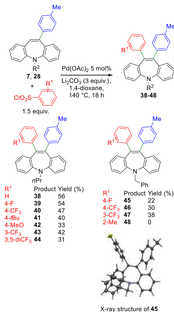
Scheme 4. Palladium-catalyzed direct C11-arylation of 10-aryl dibenzo[ b,f ]azepines with ArSO 2 Cl.
