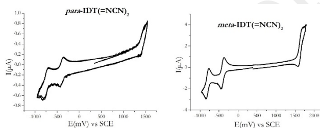
Fig. 9. CV of para -IDT(=NCN) 2 (left) and meta -IDT(=NCN) 2 (right) (10 -3 M) recorded in CH 2 Cl 2 + Bu 4 NPF 6 0.2 M, sweep-rate 100 mV.s -1 . Platinum disk (Ø: 1mm) working electrode.
