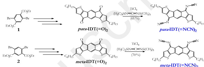
Scheme 1 Synthesis of para-IDT(=NCN) 2 (top) and meta-IDT(=NCN) 2 (bottom).
