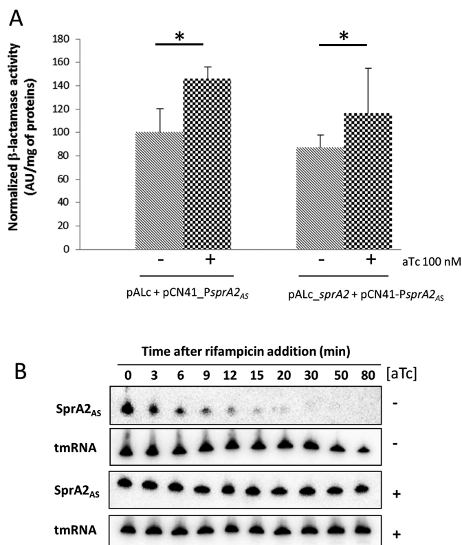
Figure 9. The presence of SprA2 affects SprA2 AS stability. (A) The effects of SprA2 on the transcriptional activity of the SprA2 AS promoter ( PsprA2 AS ). S. aureus Newman pALC and pALC_sprA2 were co-transformed with pCN41_PsprA2 AS . SprA2 expression was induced with 100 nM anhydrotetracycline (aTc) and β-lactamase activity was measured after 30 min. For each lane, the activity was normalized by subtracting the background signal from the same strain in which pCN41_PsprA2 AS was replaced by the pCN41 empty vector (not shown). The data presented are the mean of three independent experiments performed in triplicate ± standard deviation. * P < 0.05 (Mann-Whitney U test). (B) The half-life of SprA2 AS increased when SprA2 was overexpressed. S. aureus Newman strain with pALC_sprA2 + pCN35_sprA2 AS was grown in brain heart diffusion, then SprA2 expression was induced by 100 nM aTc. After 30 min, 200 μg/ml rifampicin was added to the culture, and total RNAs extracted at different time intervals. tmRNA was used as an internal loading control. The data shown are from one representative experiment out of three performed.
