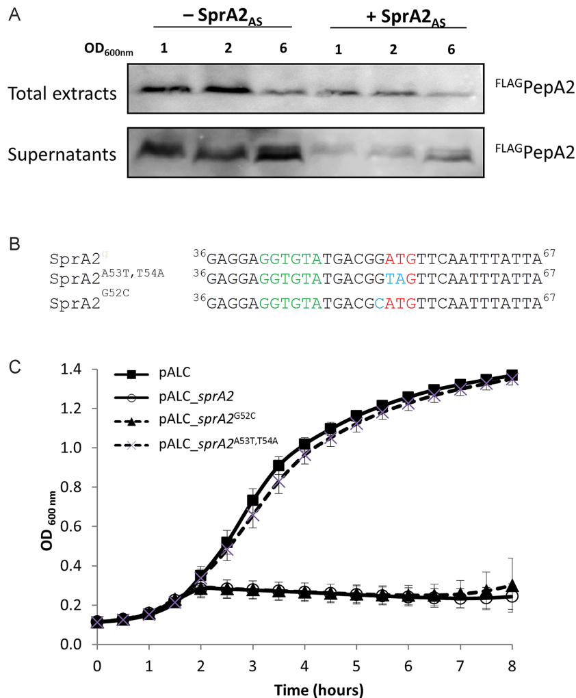
Figure 3. Bacterial toxicity is linked to the expression of PepA2. (A) In vivo expression of flagged PepA2, comparing Staphylococcus aureus Newman strains \Delta sprA2 \Delta sprA2 AS pCN35 sprA2 Flag compared to Newman \Delta sprA2 \Delta sprA2 AS pCN35 sprA2 FlagsprA2 AS . (B) Point mutations were done in sprA2 to avoid translation initiation or to modify RNA secondary structure. (C) Comparative growth curves of Newman strain containing empty plasmid pALC (squares); pALC sprA2 (circles); pALC sprA2 G52C (triangles); or pALC sprA2 A53T, T54A (crosses). Induction was done after 2 h with 1 \mu M anhydrotetracycline (aTc).
