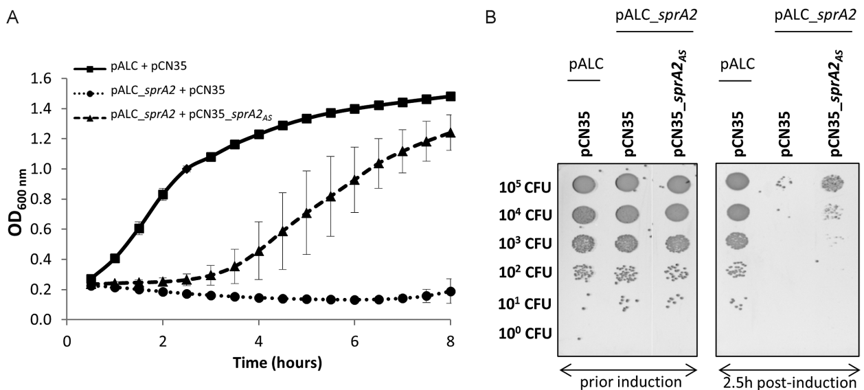
Figure 2. sprA2 / sprA2 AS encodes and expresses a functional toxin–antitoxin system. (A) Comparative growth curves after induction with 1 \mu M anhydrotetracycline (aTc) on Staphylococcus aureus Newman replicating empty plasmids pALC and pCN35 (squares); pALC_ sprA2 and pCN35 (circles); and pALC_ sprA2 and pCN35_ sprA2 AS (triangles). Growth was conducted in a Biotek instrument for 2.5 h, then expression was induced by aTc. Data points shown represent the growth after this addition, and are the mean of three independent biological replicates. (B) Assessment of cell viability by plating 10-fold serial dilutions, prior induction (left panel) or 2.5 h post-induction (right panel). All cultures (broth and agar) contain chloramphenicol and erythromycin concentrations appropriate for plasmid maintenance.
