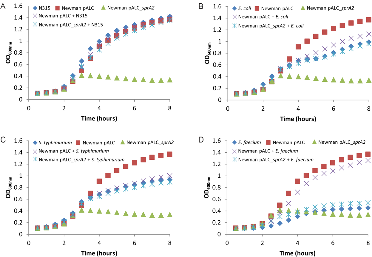
Figure 4. The SprA2 toxin does not kill other bacteria during co-cultures. (A) The effects of sprA2 expression on the growth of Staphylococcus aureus N315. Shown are: S. aureus N315 (blue diamonds); S. aureus Newman pALC (red squares); Newman pALC_ sprA2 (green triangles); Newman pALC + N315 (purple crosses); and Newman pALC_ sprA2 + N315 (blue crosses). (B) The effects of sprA2 expression on Escherichia coli growth. Shown are: E. coli EC101 (blue diamonds); S. aureus Newman pALC (red squares); Newman pALC_ sprA2 (green triangles); Newman pALC + E. coli (purple crosses); and Newman pALC_ sprA2 + E. coli (blue crosses). (C) The effects of SprA2 expression on Salmonella typhimurium growth. Shown are: S. typhimurium (blue diamonds); S. aureus Newman pALC (red squares); Newman pALC_ sprA2 (green triangles), Newman pALC + S. typhimurium (purple crosses); and Newman pALC_ sprA2 + S. typhimurium (blue crosses). (D) The effects of SprA2 expression on Enterococcus faecium growth. Shown are: E. faecium Aus004 (blue diamonds); S. aureus Newman pALC (red squares); Newman pALC_ sprA2 (green triangles); Newman pALC + E. faecium (purple crosses); and Newman pALC_ sprA2 + E. faecium (blue crosses). Growth was conducted in a Biotek instrument and 1 \mu M aTc was added after 2.5 h. The data presented are the mean of three independent experiments performed in triplicate. To improve readability, the standard deviations (which never exceeded 0.057) were omitted.
