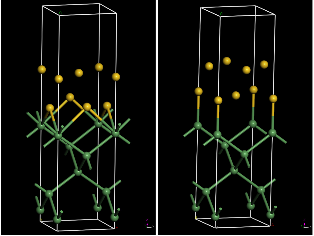
FIG. 4. (color online) 3D view for \text{Ge}(001)/\sqrt{2} \times \sqrt{2}\text{R}45^\circ\text{-Au}(001) models. Left panel: Top-Hollow (tH). Right panel: Bridge-Bridge (BB). To increase visibility only two Au-layers and five Ge-layers are shown.
