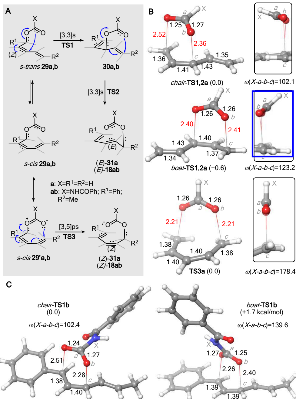
Figure 10. (A) Sequential vs. one-step (3,3) and (3,5) dioxa-rearrangements of model esters ( Z )- 29a,b to yield ( E )- 31a,b and ( Z )- 31a,b . (B) Optimized geometries (B3LYP-D3(PCM=CHCl 3 )/6-311++G(d,p) level of theory) and relative energies of transition structures chair-TS1,2a , boat-TS1,2a and TS3a . (C) Chief geometric and energetic features (B3LYP-D3(PCM=CHCl 3 )/6-311++G(d,p)/B3LYP/6-31G(d) level of theory) of transition structures chair-TS1b and boat-TS1b . Bond distances are given in Å. Numbers in parentheses are the relative energies, in kcal/mol. The dihedral angle \omega (in deg.) is defined by the X-a-b-c atoms.
