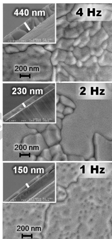
Figure 12: SEM images of thin films deposited at different laser-pulse repetition rates. All the experiments were performed with the substrates temperature at 600 °C, target-substrate distance of 55 mm and oxygen pressure of 0.5 mbar. The details show the film thickness.
