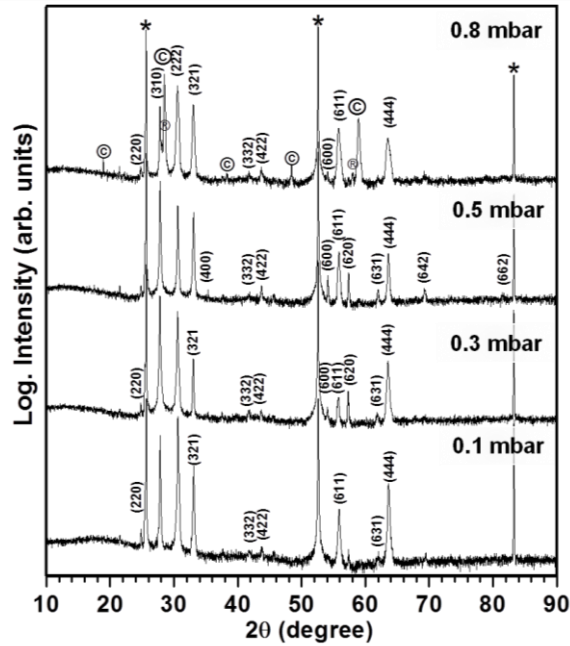
Figure 07: X-ray patterns of thin films deposited on substrates at different oxygen pressures. All the experiments were performed at constant laser-pulse repetition rate of 2 Hz, target-substrate distance of 55 mm and substrate temperature of 600 °C. The \gamma - \text{Bi}_{12}\text{TiO}_{20} phase is assigned with the Miller indexes and the metastable phase is indicated by ©. The peaks assigned with * belong to substrate.
