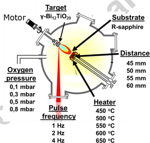
Figure 01: Experimental parameters used to obtain the BTO thin films by PLD. The films were deposited on substrates of R-sapphire at different temperatures, evaluating the influence of the oxygen pressure, the distance between the target and the substrate and the laser-pulse repetition frequency. All the depositions occurred during 15 minutes.
