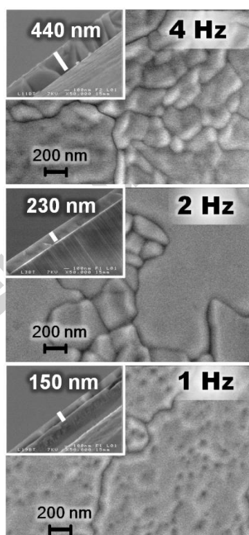
Figure 12: SEM images of thin films deposited at different at different laser-pulse repetition rates. All the experiments were performed with the substrates temperature at 600 °C, target-substrate distance of 55 mm and oxygen pressure of 0.5 mbar. The details show the film thickness.
