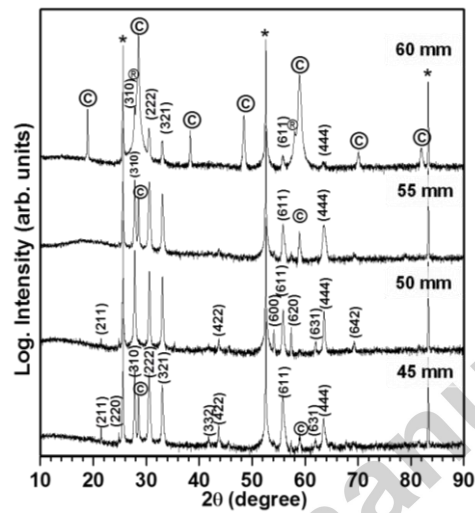
Figure 09: X-ray patterns of thin films deposited on substrates at different target-substrate distances. All the experiments were performed at constant laser-pulse repetition rate of 2 Hz, substrate temperature of 600 °C and oxygen pressure of 0.5 mbar. The \gamma - \text{Bi}_{12}\text{TiO}_{20} phase is assigned with the Miller indexes and the metastable phase is indicated by ©. The peaks assigned with * belong to substrate.
