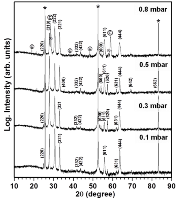
Figure 07: X-ray patterns of thin films deposited on substrates at different oxygen pressures. All the experiments were performed at constant laser-pulse repetition rate of 2 Hz, target-substrate distance of 55 mm and substrate temperature of 600 °C. The \gamma - \text{Bi}_{12}\text{TiO}_{20} phase is assigned with the Miller indexes and the metastable phase is indicated by ©. The peaks assigned with * belong to substrate.
