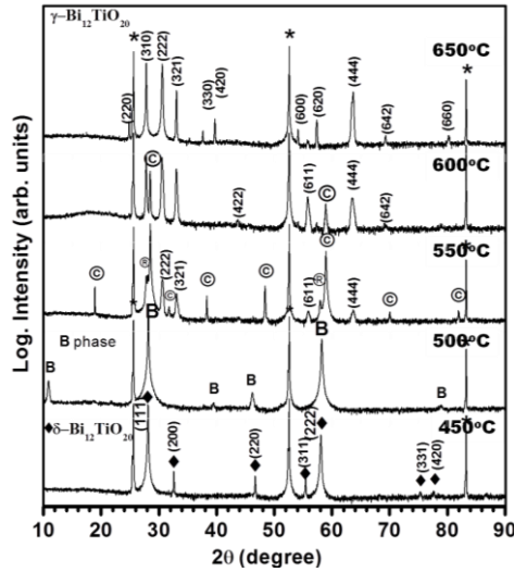
Figure 02: X-ray patterns of thin films deposited on substrates at different temperatures. All the experiments were performed at constant laser-pulse repetition rate of 2 Hz, oxygen pressure of 0.5 mbar and target-substrate distance of 55 mm. The \delta - \text{Bi}_{12}\text{TiO}_{20} phase is assigned with ♦. Unknown BTO phases are assigned by B, © and ® and the peaks assigned with * belong to the substrate.
