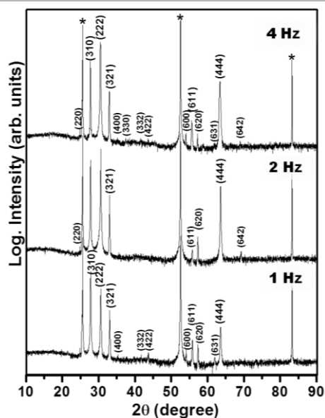
Figure 11: X-ray patterns of thin films deposited on substrates at different laser-pulse repetition rates. All the experiments were performed with the substrates temperature at 600 °C, target-substrate distance of 55 mm and oxygen pressure of 0.3 mbar. The \gamma - \text{Bi}_{12}\text{TiO}_{20} phase is assigned with the Miller indexes and the metastable phase is indicated by ©. The peaks assigned with * belong to substrate.
