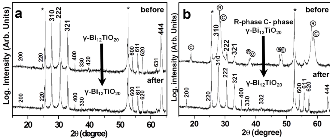
Figure 03: X-ray patterns of the BTO thin films before and after annealing at 700 °C for 2 hours. The XRD patterns in (a) show that thermodynamically stable \gamma - \text{Bi}_{12}\text{TiO}_{20} is unaffected the annealing, while the metastable phases (b) are transformed to the \gamma - \text{Bi}_{12}\text{TiO}_{20} phase after the treatment.
