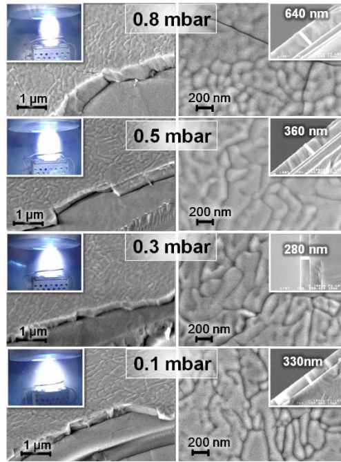
Figure 08: SEM images of thin films deposited at different oxygen pressures. All the experiments were performed at constant laser-pulse repetition rate of 2 Hz, target-substrate distance of 50 mm and substrate temperature of 600 °C. The details show the respective plasma plume and the film thickness.
