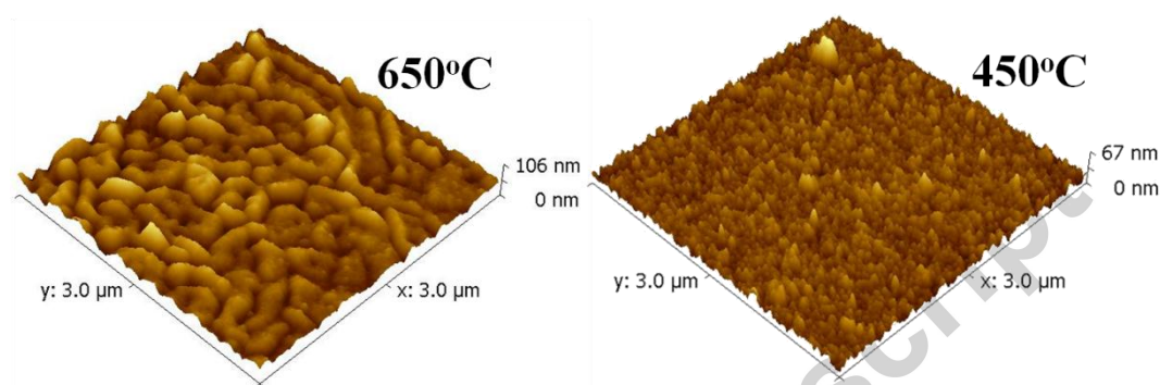
Figure 6: AFM images of the \text{Bi}_{12}\text{TiO}_{20} thin films deposited at 650 °C and 450 °C. The experiments were performed at constant laser-pulse repetition rate of 2 Hz, oxygen pressure of 0.5 mbar and target-substrate distance of 50 mm.
