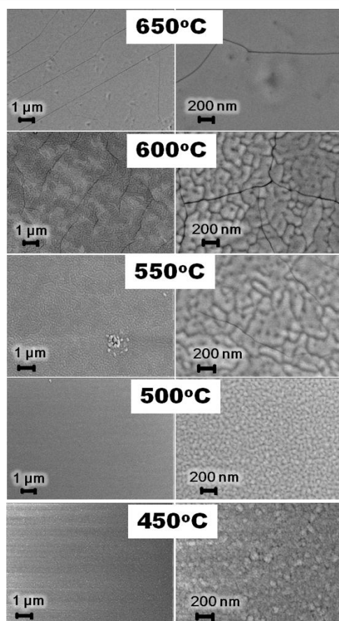
Figure 05: SEM images of the films deposited on the substrate at different temperatures. All the experiments were performed at constant laser-pulse repetition rate of 2 Hz, oxygen pressure of 0.5 mbar and a target-substrate distance of 55 mm.
