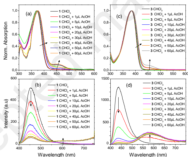
Figure 9. Steady state absorption (a) and (c) and fluorescence (b) and (d) spectra of 1 and 3 upon addition of various amounts of AcOH in 3 ml \text{CHCl}_3 solutions ( 2.5 \times 10^{-6} \text{M} ). The excitation wavelength for the fluorescence spectra was 380 nm. The arrows show the change of the spectra by increasing the amount of AcOH.
