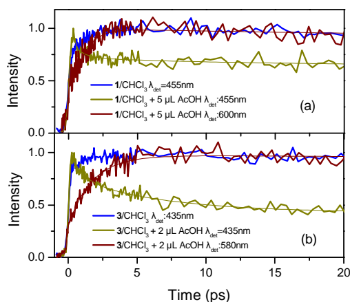
Figure 10. Fluorescence dynamics for (a) 1 and (b) 3 in \text{CHCl}_3 within the first 20 ps, with and without AcOH, at emission wavelengths corresponding to the fluorescence bands of the neutral and protonated species. exc. 385 nm.
