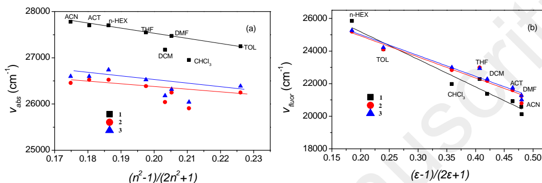
Figure 3. Plot of the solvent shift of absorption (a) and fluorescence (b) peak of the compounds 1 , 2 and 3 as a function of f(n^2) = (n^2 - 1)/(2n^2 + 1) and f(\epsilon) = (\epsilon - 1)/(2\epsilon + 1) , respectively.
