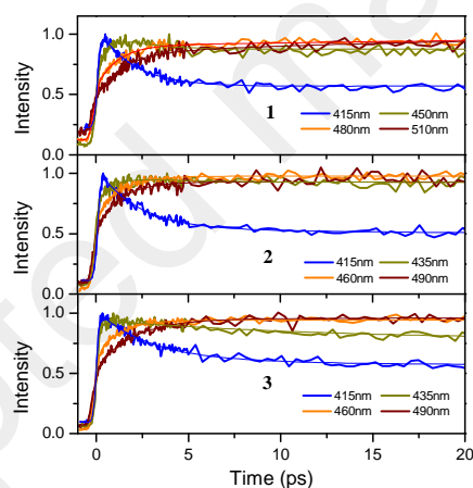
Figure 7. Fluorescence dynamics within the first 20 ps for 1 , 2 and 3 in THF at various detection wavelengths. exc. 385 nm.
