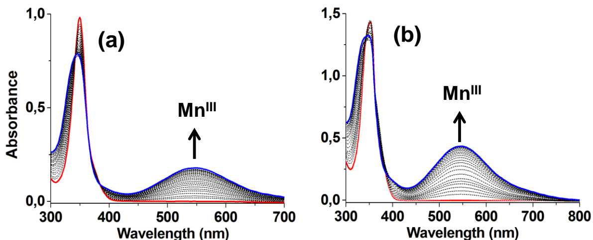
Figure 4. Time-resolved UV-vis spectral changes observed during irradiation at 400 nm of aerobic solutions in DMF at 20 °C of (a) 1 from 0 - 70 min, c = 30 \mu\text{M} , d = 0.5 \text{ cm} , and (b) 2 from 0 – 34 min, c = 300 \mu\text{M} , d = 0.2 \text{ cm} .
