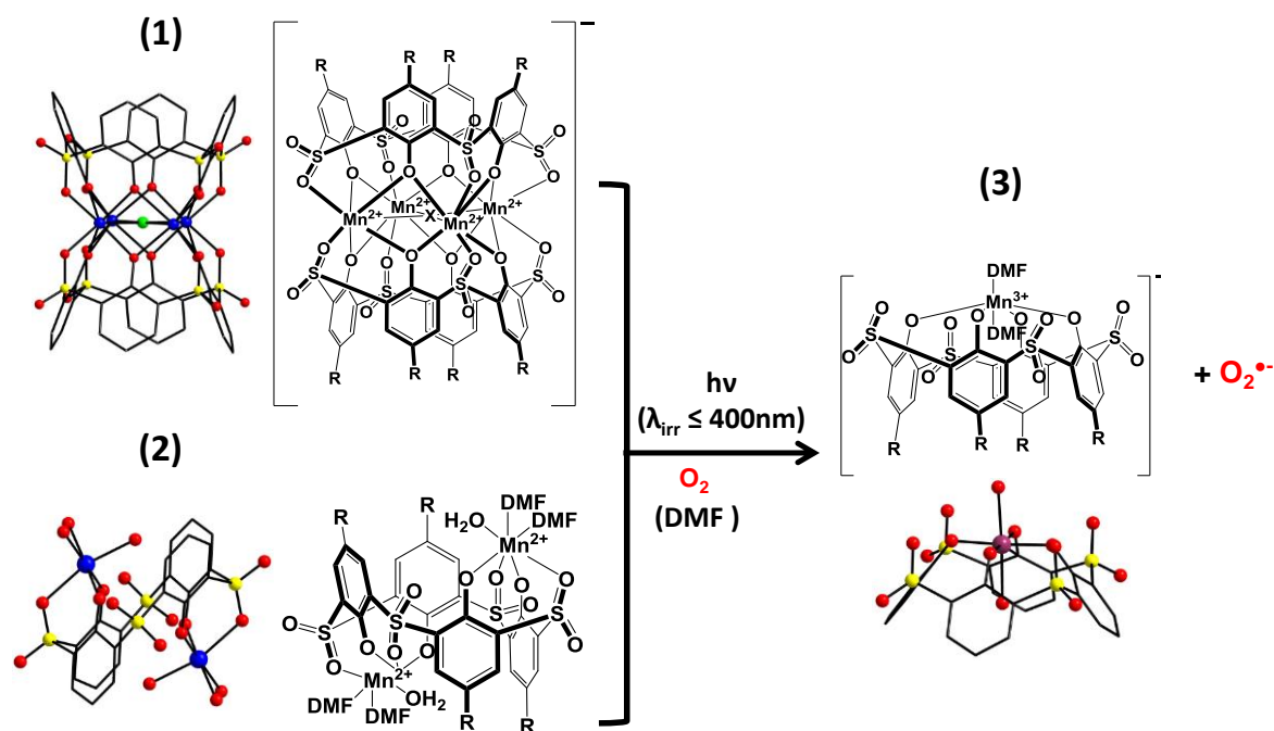
Scheme 1. Photo-reactivity of compounds 1 and 2. R = tert -butyl or H. Each atom is depicted as follows: \text{Mn}^{2+} , blue; \text{Mn}^{3+} , violet; S, yellow; O, red.
