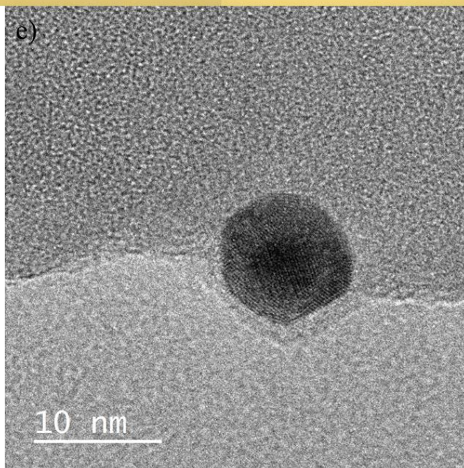
Figure 1: a) Pristine quenched glass; b) Sintered glass; c) Sample containing 0.01 % w of gold; d) Sample containing 0.2 % w of gold; e) TEM image of a GNP coated on the glass.
