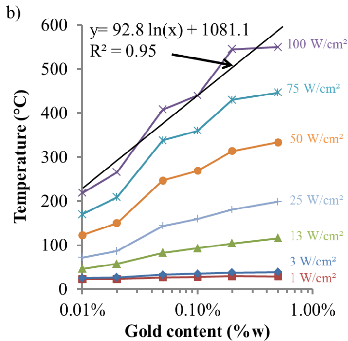
Figure 3: a) Evolution of the temperature with the laser power for different gold content (in weight percent); b) Increase of the temperature as a function of the gold content for different laser powers.
