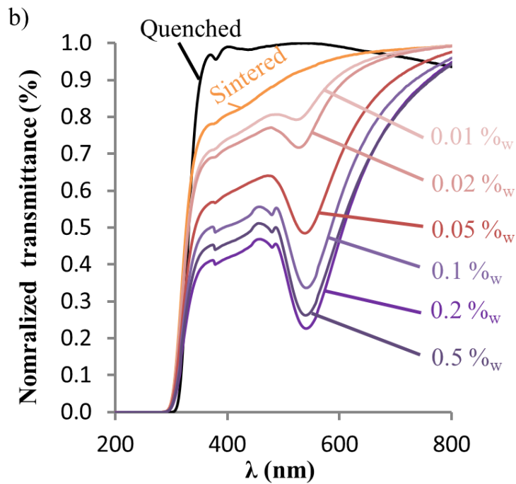
Figure 2: a) Transmittance in the visible range of the different composites and glass between 200 and 800 nm; b) Normalized transmittance in the visible range of the different composites and glass between 200 and 800 nm.
