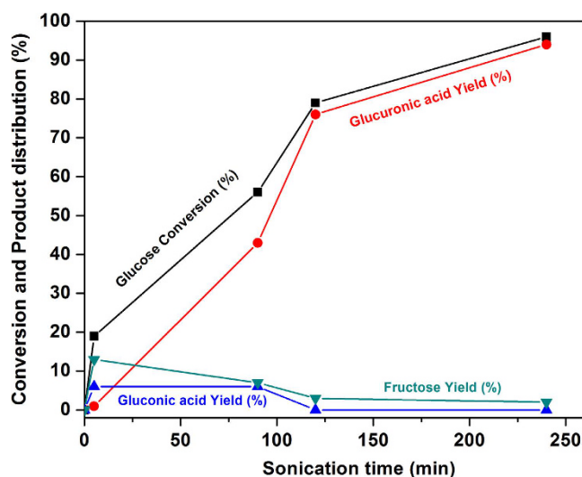
Figure 3. Kinetic profile of the glucose oxidation under high frequency ultrasound (2 g of glucose in 100 mL of H 2 O, 25 °C, 100 rpm stirring, ultrasonic irradiation (550 kHz, P_{\text{acous}} = 0.36 \text{ W.mL}^{-1} ).
