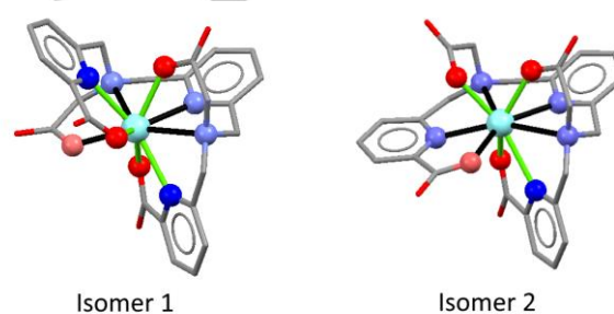
Figure 2. Representation of the DFT optimized geometry of the two isomers of [YL 5 ]. Donor atoms belonging to the pseudo-equatorial plane represented in light colours with black bonds to the Yttrium (light blue). Other coordination bonds are depicted in green.
