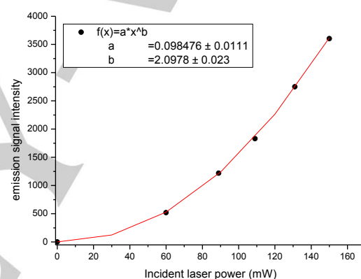
Figure 8. Variation of the Eu(III) luminescence intensity with the laser excitation of [\text{EuL}^{5\text{c}}]^{4+} in water (2P-excitation \lambda_{\text{ex}} = 760 \text{ nm} , \bullet ). The red line represents the fitting of the experimental points by the polynomial function indicated in inset.
