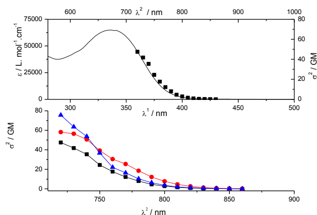
Figure 9. (Top) 1P-absorption spectrum of [\text{EuL}^{5c}]^{4+} in water at RT (black line, lower abscissa). Superimposed on this plot is the 2P-absorption measured by TPEF method in water in wavelength doubled scale ( \blacksquare , upper abscissa). (bottom) 2P-absorption spectra of [\text{EuL}^{5c}]^{4+} ( \blacksquare ), [\text{EuL}^{5d}]^{6-} ( \blacktriangle ) to [\text{EuL}^{5e}]^{8-} ( \bullet ).
