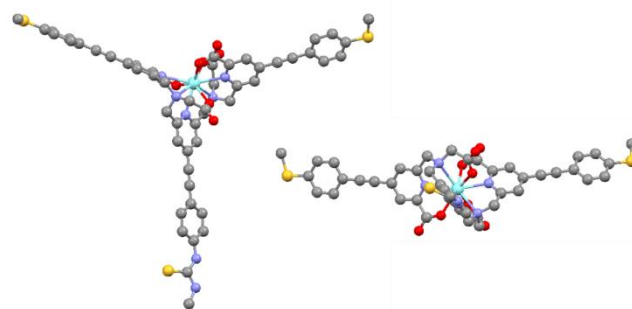
Figure 3. Representation of the DFT optimized geometry of the isomers 1 of [YL 5c ].
