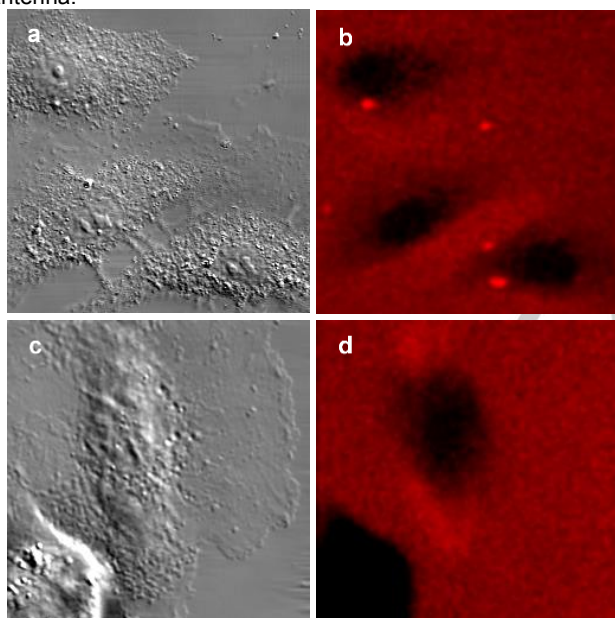
Figure 10. 2P imaging of living T24-cells stained with [\text{EuL}^{5c1}]^{4+} (b) and [\text{EuL}^{5e1}]^{8-} (d). ( \lambda_{\text{exc}} = 780 \text{ nm} ). In (a) and (c) the corresponding transmitted light DIC images are represented. Complexes are added in the cell medium in phosphate buffer solution to reach a final concentration of 5\text{-}10 \cdot 10^{-6} \text{ mol.L}^{-1} .
