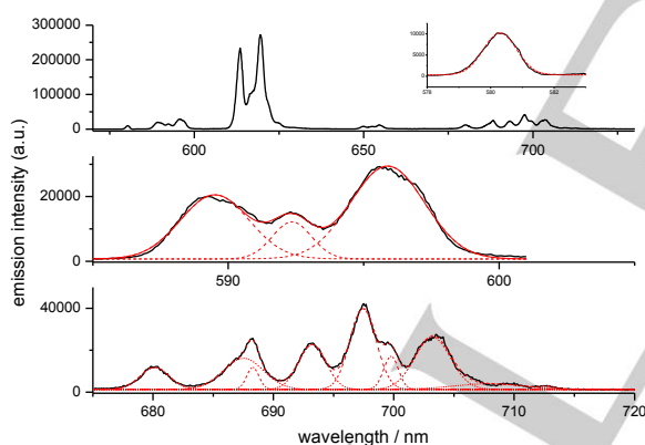
Figure 6. 77K emission spectra of [\text{EuL}^{5c}]^{4+} (black) in organic glass (MeOH/EtOH, 1/4, v/v) under 370 nm excitation with optimal resolution (detection slit 0.2, increment 0.2 nm). (Top) full spectra, in inset is represented the magnification of the J=0 transition emission spectrum with a single Gaussian deconvolution (red). (Middle) Magnification of the J=1 transition and decomposition in three Gaussian curves (dashed red, sum in red). (Bottom) Magnification of the J=4 transition and decomposition in nine Gaussian curves (dashed red, sum in red).
