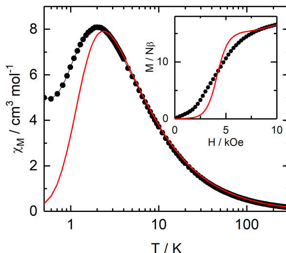
Figure 2. Thermal variation of the magnetic susceptibility in black dots with the calculated one (red line) according to the model developed in main text; (inset) Field variation of the magnetization at 500 mK and the calculated curve (red line).
