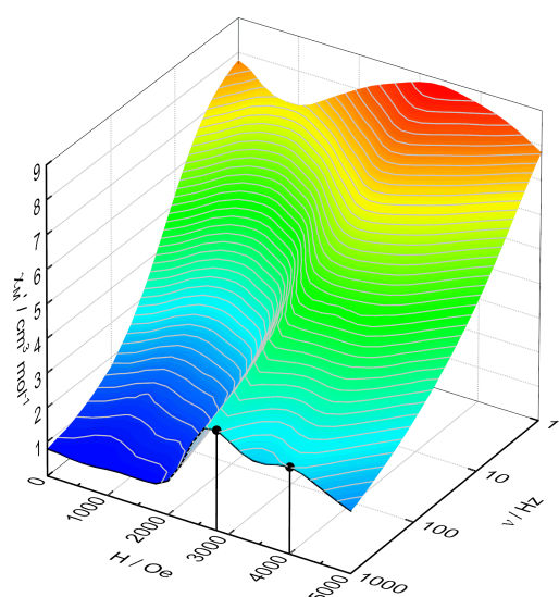
Figure 6. Variation of the in-phase component ( \chi_M' ) at 2 K with the frequency of the oscillating field ( \nu ) and the external dc field ( H ). The thick black line corresponds to \chi_M' values at 1000 Hz and the two dots to the observed maxima at 2.8 and 4 kOe.
