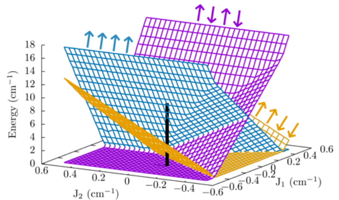
Figure 4. EES for states |\uparrow\downarrow\uparrow\downarrow\rangle , |\uparrow\uparrow\downarrow\downarrow\rangle and |\uparrow\uparrow\uparrow\uparrow\rangle . State |\uparrow\downarrow\uparrow\downarrow\rangle has been omitted for clarity. The vertical black segment corresponds to the best agreement with the experiment ( J_1 = -0.27 \text{cm}^{-1} and J_2 = -0.09 \text{cm}^{-1} ).
