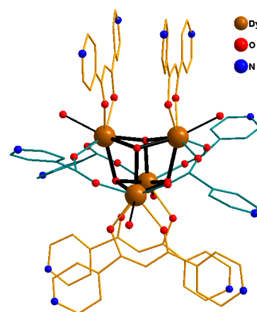
Figure 1. Representation of the crystal structure of Dy 4 . BppdH are in yellow rods, PaH in green rods, while Dy, O and N are in gold, red and blue balls, respectively. Hydrogen atoms have been omitted for clarity.
