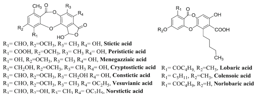
Fig. 9 Structure of depsidones isolated from Stereocaulon species
