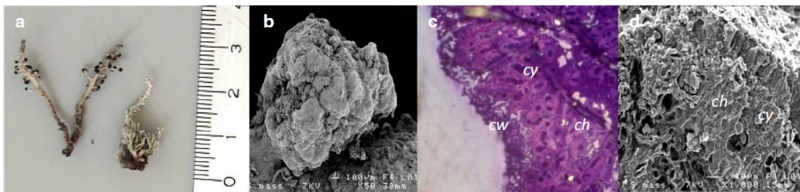
Fig. 7 S. halei . a General morphology, b detail of an external cephalodium (SEM, \times 25 ) cd transversal section of a protosacculate cephalodium (light microscopy, \times 400 , HES coloration
