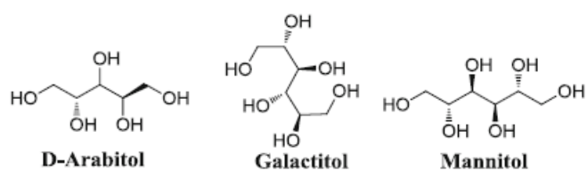
Fig. 15 Structure of polyols isolated from Stereocaulon species
