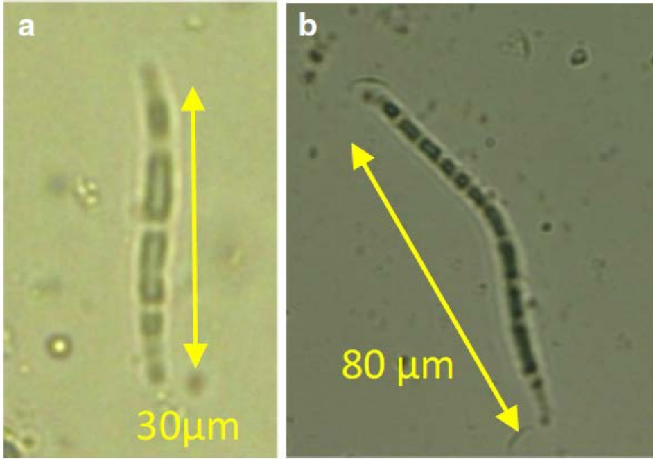
Fig. 5 Morphology of spores. a Fusiform for S. halei , b vermiform for S. montagneanum (see supplementary data M1)
