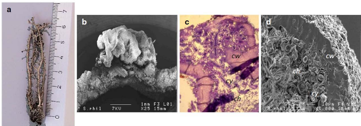
Fig. 6 S. montagneanum . a General morphology, b detail of an external cephalodium (SEM, \times 25 ) cd transversal section of a sacculate cephalodium (light microscopy, \times 400 , HES
