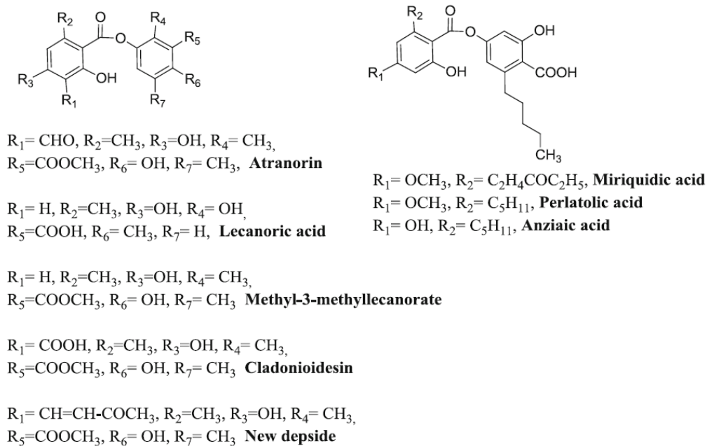
Fig. 8 Structure of depsides isolated from Stereocaulon species
