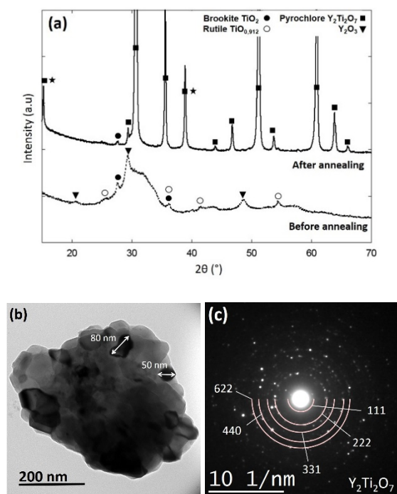
Figure 4 : (a) X-ray diffraction patterns of ball-milled powder before and after annealing at 900^\circ\text{C} . (b) TEM micrograph of powder after annealing at 900^\circ\text{C} and (c) SAED pattern of the same sample
