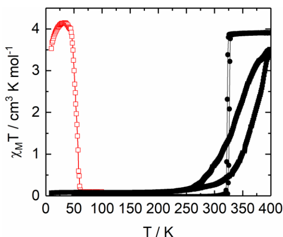
Figure 6. Thermal dependence of \chi_M T for 1 (full circles), 1-4MeNO 2 (full square). The thermal dependence of \chi_M T 1-4MeNO 2 after light irradiation (660 nm, 5 mW) is represented with red squares.
