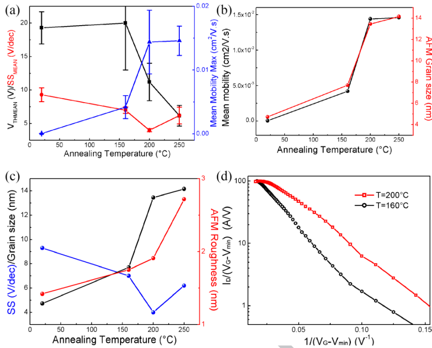
Fig.5: (a) Behavior of the mean threshold voltage V_{THMEAN} , subthreshold slope SS_{MEAN} and field effect mobility, when the annealing temperature increases; (b) Similar behavior of the mobility and the grain size as a function of the annealing temperature; (c) Behavior of the subthreshold slope SS , the surface roughness and the grain size as a function of the annealing temperature; (d) Semi-logarithmic plot of I_D/(V_G-V_{min}) versus 1/(V_G-V_{min}) for OFETs annealed at 160°C and 200°C
