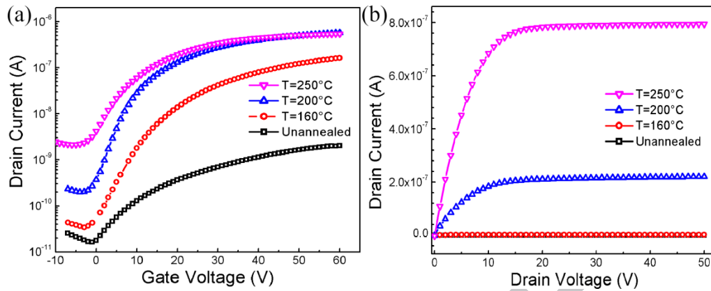
Fig.4: (a) Mean transfer characteristics ( V_D=20\text{V} ) and (b) output characteristics ( V_G=20\text{V} ) of several OFETs having the same size (channel width W=4000\ \mu\text{m} , channel length L=150\ \mu\text{m} ) and 125 nm thick C_{60} active layer, measured as-fabricated and after annealing at 160°C, 200°C and 250°C.
