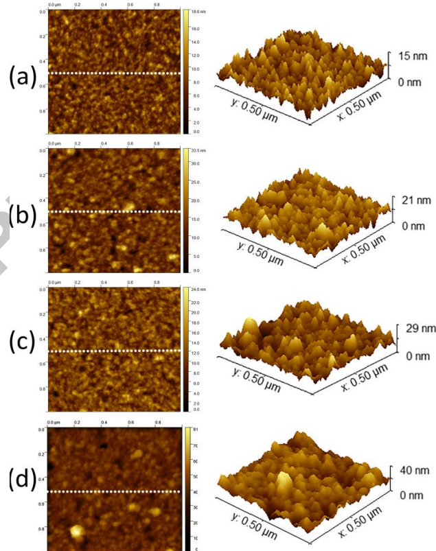
Fig. 3: 2D ( 1 \times 1 \mu\text{m}^2 ) AFM images, corresponding 3D enlarged ( 0.5 \times 0.5 \mu\text{m}^2 ) (a) as-deposited; and after annealing at 160°C (b), 200°C (c) and 250°C (d)
