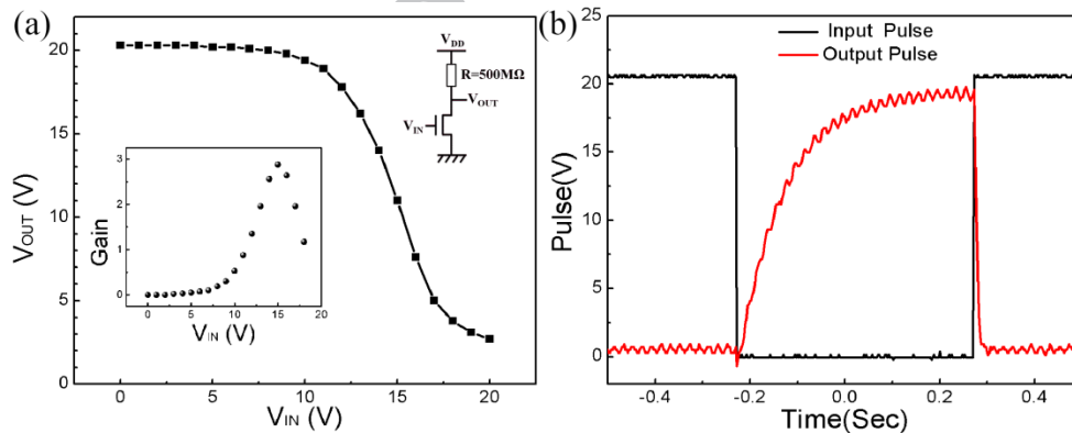
Fig. 7: (a) Static output characteristic of printed C_{60} based OFET loaded by 500\text{M}\Omega resistance and (b) its response to 1Hz pulse. The inset shows the gain of the inverter with a maximum value of 3.
