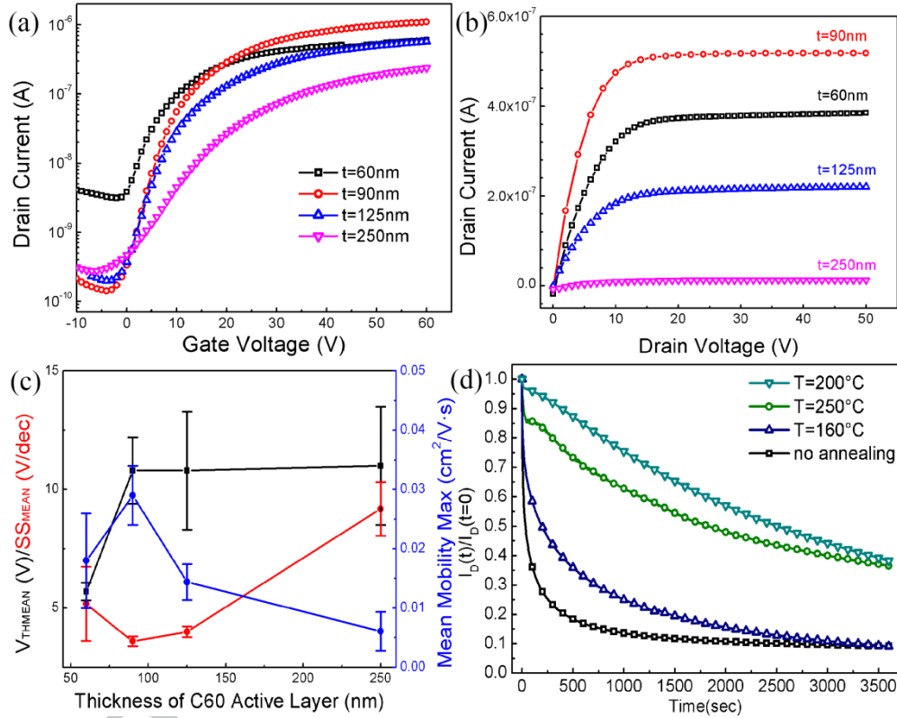
Fig. 6: (a), (b), (c): Mean transfer and output characteristics of several OFETs having the same size (channel width W=4000 \mu\text{m} , channel length L=150 \mu\text{m} ) and a C_{60} active layer with a thickness of 60nm, 90 nm, 125 nm or 250nm. The behavior of their mean electrical parameters (Threshold voltage, subthreshold slope and mobility) is also reported. (d) Drain-current of OFETs using 90 nm thick C_{60} active layer un-annealed and annealed at different temperatures, 160°C, 200°C, 250°C as a function of the time under 40V gate-source voltage and 20V drain-source voltage
