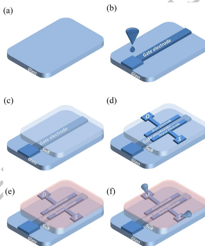
Fig. 2: Fabrication process of \text{C}_{60} OFET
