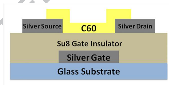
Fig. 1: Cross-section of the C_{60} OFETs using bottom gate and bottom contacts geometry. The figure highlights the problematic of the high aspect ratio between the drain and source contacts and the gate insulator
