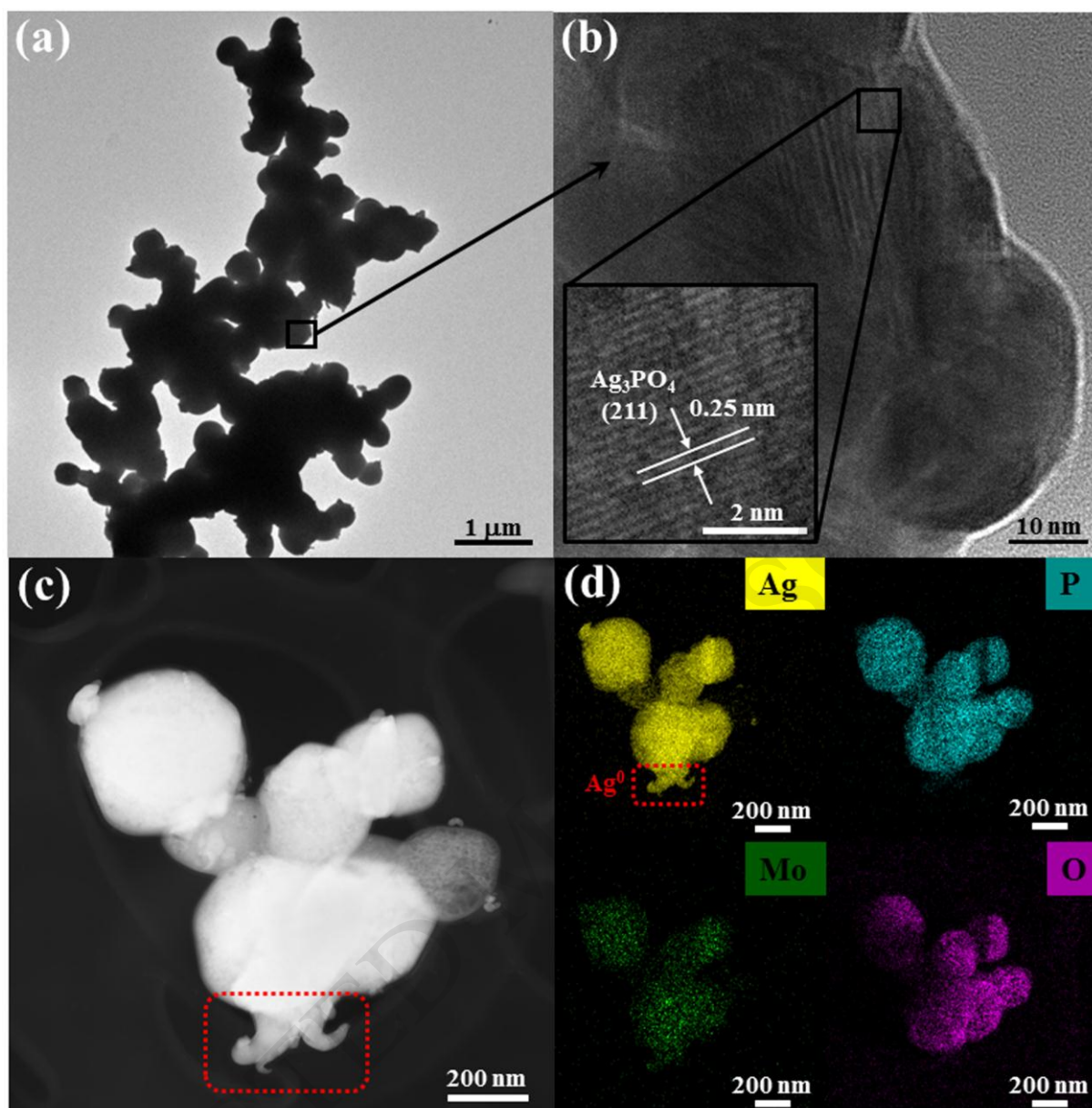
Figure 6. TEM images of (a) \text{Ag}_3\text{PO}_4:\text{Mo} 2%, (b) characteristic interplanar distance of \text{Ag}_3\text{PO}_4 , (c) and (d) EDS maps of a group of particles in \text{Ag}_3\text{PO}_4:\text{Mo} 2%.
