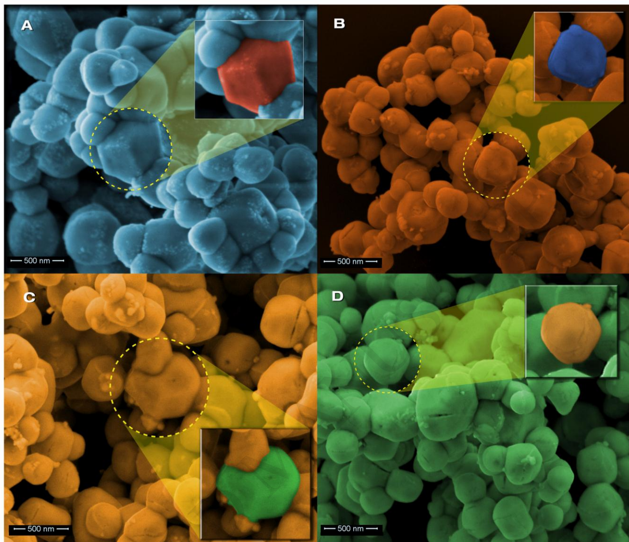
Figure 5. FEG-SEM images of (a) Ag 3 PO 4 , (b) Ag 3 PO 4 /Mo 0.5%, (c) Ag 3 PO 4 /Mo 1% and (d) Ag 3 PO 4 /Mo 2%.
