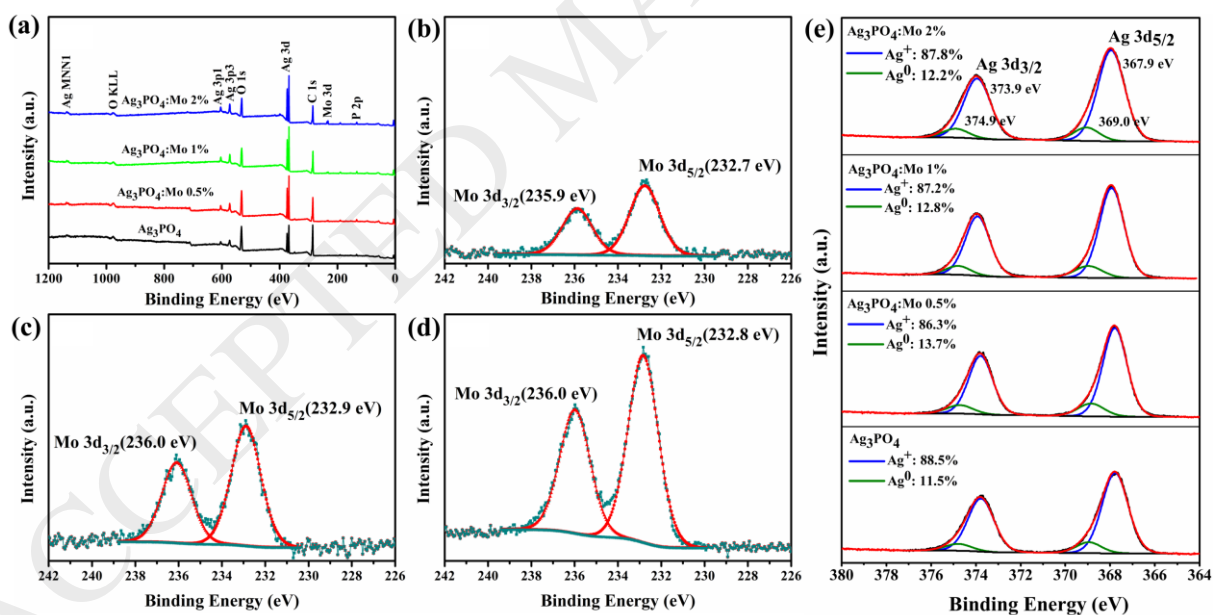
Figure 4. XPS survey spectra of pure (black line) and \text{Mo}^{6+} doped (increasing amount from the bottom to top) \text{Ag}_3\text{PO}_4 microcrystals (a) and XPS spectrum of Mo 3d for \text{Ag}_3\text{PO}_4:\text{Mo} 0.5% (b), \text{Ag}_3\text{PO}_4:\text{Mo} 1% (c), \text{Ag}_3\text{PO}_4:\text{Mo} 2% (d) samples and (e) XPS spectra of Ag 3d for \text{Ag}_3\text{PO}_4 , \text{Ag}_3\text{PO}_4:\text{Mo} 0.5%, \text{Ag}_3\text{PO}_4:\text{Mo} 1% and \text{Ag}_3\text{PO}_4:\text{Mo} 2% samples.
