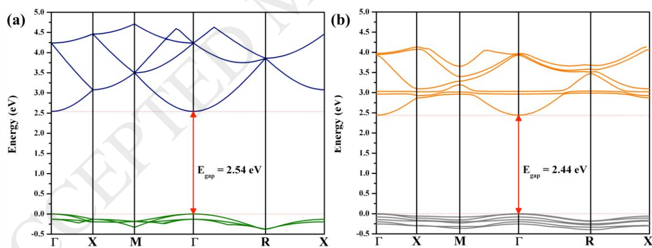
Figure 8. The band structure of pure Ag 3 PO 4 and Ag 3 PO 4 :Mo supercells.
