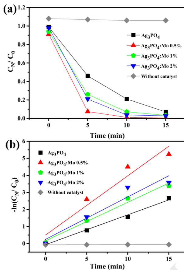
Figure 12. Photocatalytic degradation of RhB ( 1.0 \times 10^{-5} mol L -1 ) in the absence and in the presence of Ag 3 PO 4 and Ag 3 PO 4 doped with different amounts of Mo in linear plot (a) and in log plot for the determination of the rate constant (b).
