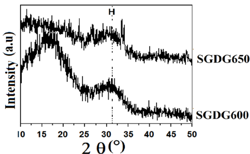
Fig. 1. X-ray diffraction patterns of SGDGDG heated at 600°C and 650°C.
