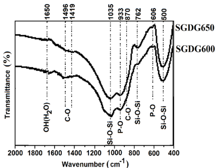
Fig. 2. FTIR spectra of SGD glass heated at 600°C and 650°C.
