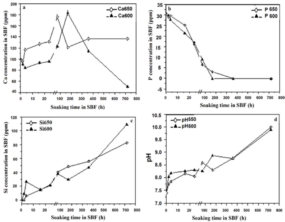
Fig. 3. Evolutions of Ca (a), P (b) and Si (c) concentrations in SBF, and evolution of SBF pH (d), versus soaking time of SGDGD heated at 600°C and 650°C.
