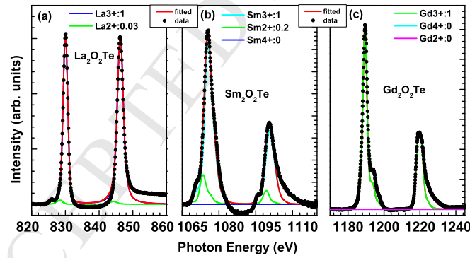
Figure 2: (Color online) Normalized NEXAFS spectra at (a) La M_{5,4} -edge for La_2O_2Te , (b) Sm M_{5,4} -edge for Sm_2O_2Te , and (c) Gd M_{5,4} -edge for Gd_2O_2Te .
