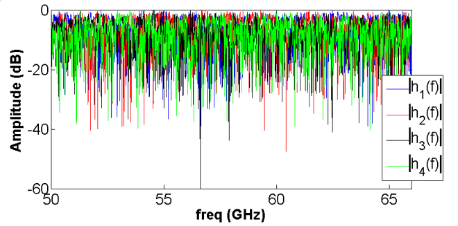
Fig. 5. Absolute value [dB] of the measured transfer functions by means of a VNA along the frequency band.
