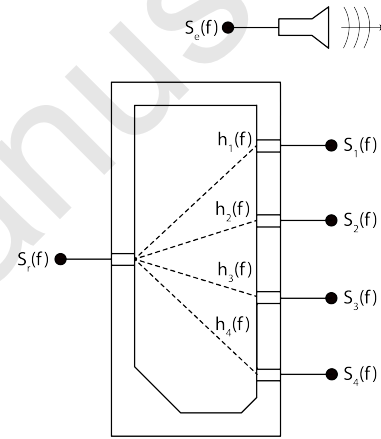
Fig. 1. Cutting view drawing of the 1x4 passive device with the associated transfer functions h_m(f) for m = 1, \dots, 4 .
