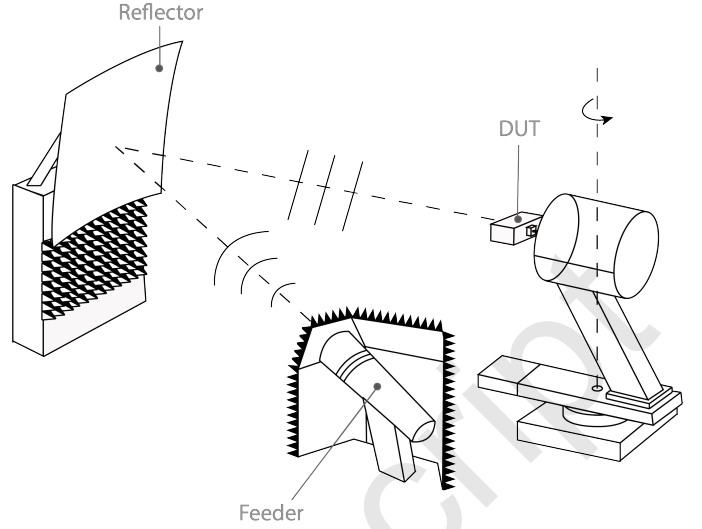
Fig. 8. Setup measurement by using a compact antenna test range.
