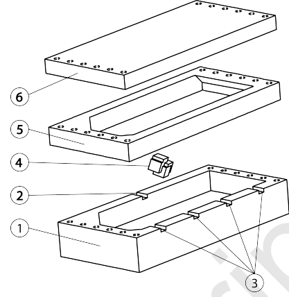
Fig. 2. Exploded view drawing of the passive device with 1) the lower part with 2) the input and 3) the output ports. 4) the diffractive element at the center of the cavity and 5/6) the upper parts closing the cavity.
