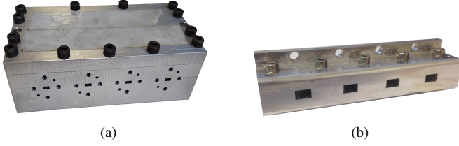
Fig. 3. Photography of (a) the output face of the realized PCD, which works at millimeter-waves, and (b) the front-end horn antenna module.
