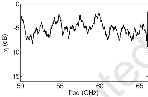
Fig. 7. Measured power efficiency of the passive device, which corresponds to the outgoing powers from the four ports versus the incoming power, along the frequency.
