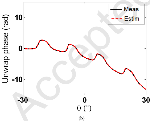
Fig. 11. Measured data at f_0 = 50 GHz (a) |S_r(\theta, f_0)| [dB] and (b) \arg(S_r(\theta, f_0)) [rad]. The black line corresponds to the normalized measured data ( S_r(\theta, f) ) and the dashed red line corresponds to the normalized estimated data model by using the estimated transfer function found from the minimization procedure ( \hat{S}_r(\theta, f) ).
