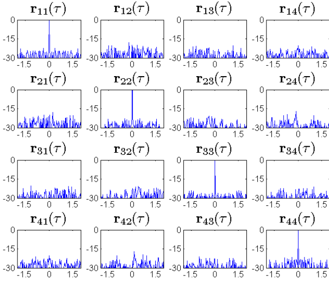
Fig. 6. r_{ij}(\tau) = DFT^{-1}[h_i(f)h_j(f)^*] , the time-domain correlation results between the measured transfer functions (VNA measurements), with the time domain \tau [ns] along the horizontal axis and the normalized amplitude [dB] along the vertical axis.
