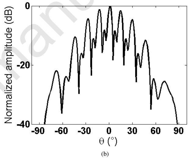
Fig. 10. Normalized measured data along (a) |S_r(\theta, f)| [dB] (b) |S_r(\theta, f_0)| [GHz] with f_0 = f + f_c = 50 GHz.
