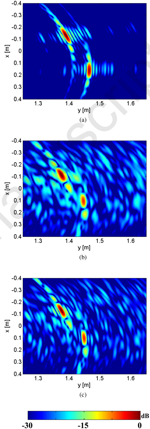
Fig. 16. Measurement imaging results using Eq. (13), of two isotropic targets (corner reflectors) captured by (a) a classic SIMO configuration with 1Tx (transmitting element) and 40 Rx (receiving elements), (b) the PCD with 10 Rx elements where the Port-to-Port measurement is used to have the transfer function, and (c) the PCD with 10 Rx elements where the plane-wave estimation is used to have the transfer function.
