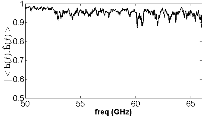
Fig. 13. Amplitude of the normalized inner product results between \mathbf{h}(f) and \hat{\mathbf{h}}(f) , along the frequency.
