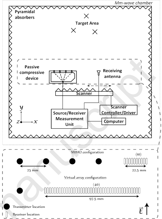
Fig. 14. Measurement setup.
