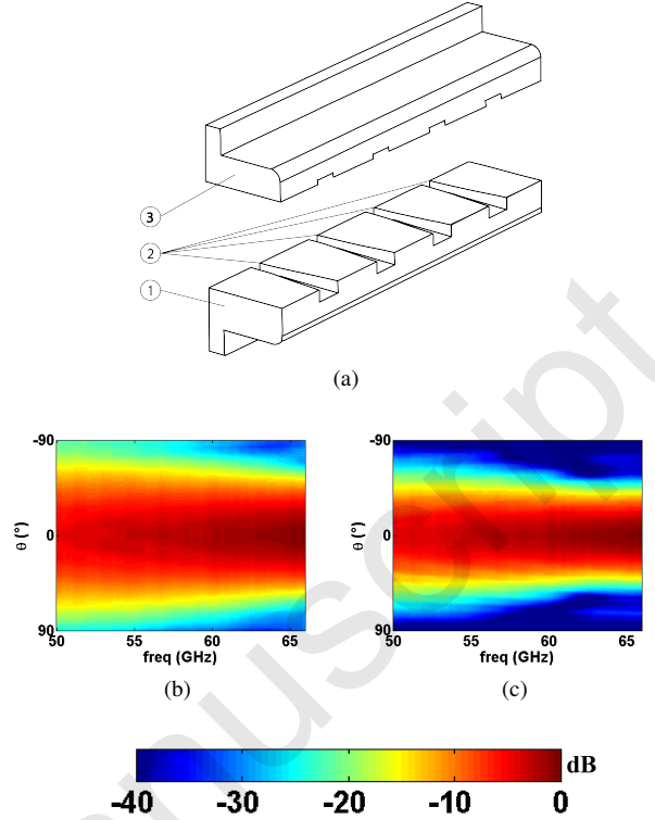
Fig. 4. Details of the antenna module with four similar horn antennas with a 8 \times 5 \text{ mm}^2 aperture size (a) Exploded view drawing of the horn antenna module with 1) the lower part, 2) the input ports attached to the output ports of the PCD, 3) the upper part. The measured radiation pattern of the first port along (b) the E-plane Co-polar and (c) H-plane Co-polar ( G(\theta, f) ).
