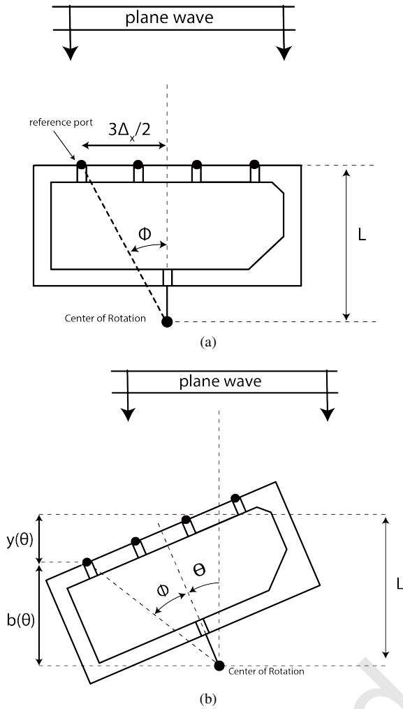
Fig. 9. Sketch of the phase variation that occurs when the DUT is looking (a) broadside and (b) at squint angle.
