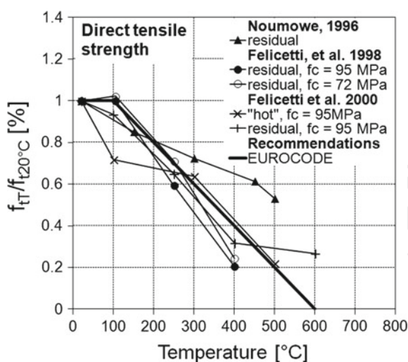
Fig. 5.59 Relative direct tensile strength test results
