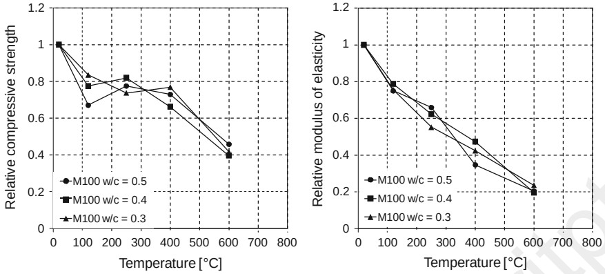
Fig. 5.13 Compressive strength (left) and modulus of elasticity (right) of HPC made with different w/c-ratios (but same mix composition) according to Hager and Pimienta (2004b)
