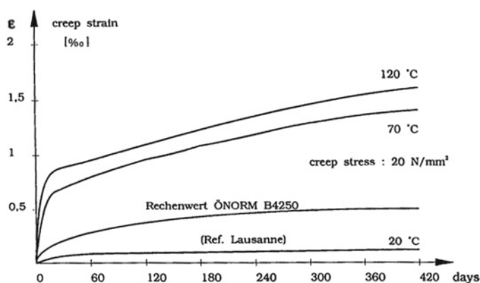
Fig. 5.24 Basic creep of high performance basalt concrete; samples tested in autoclave (concrete tested at age of 90 days) (Schneider 1982)
