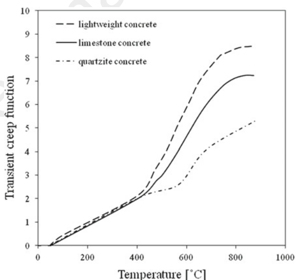
Fig. 5.46 Transient thermal strains (transient creep—Schneider's nomenclature) of concretes with different type of aggregates (Schneider 1988)
