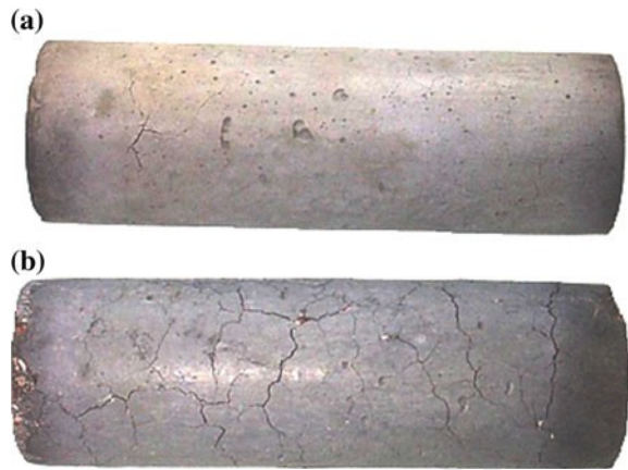
Fig. 5.41 Visible cracks on the surface of specimens after heating to 600 °C, a HPC with calcareous, and b HPC with silico-calcareous aggregates
