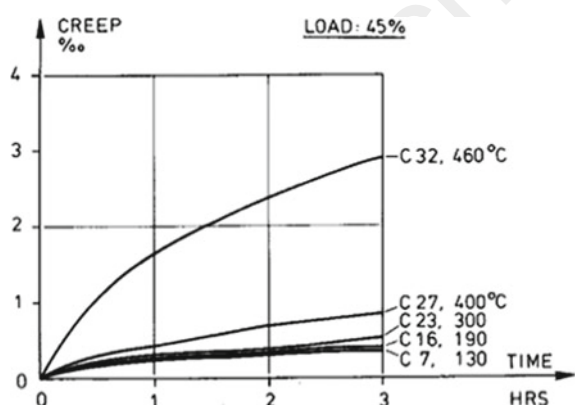
Fig. 5.30 Drying creep of concrete load level 45% (Anderberg and Thelandersson 1976)
