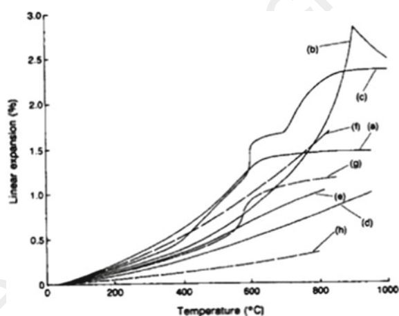
Fig. 5.37 Thermal strain of aggregates; a and g—sandstone, b and f—calcareous, c—granite, d—orthosite, e—basalt and h—pumice (Bažant and Kaplan 1996)
