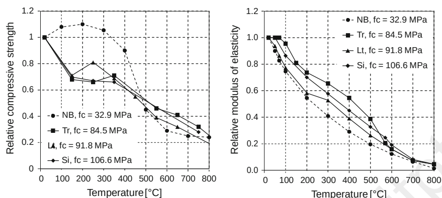
Fig. 5.2 Relative compressive strength (left) and modulus of elasticity (right) of normal and high strength concrete according to Diederichs et al. (1989)
