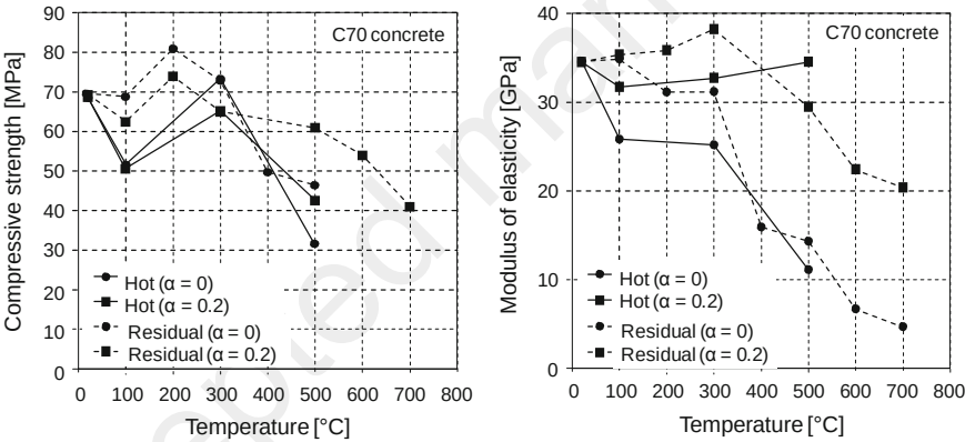
Fig. 5.23 Comparison of the “hot” and “residual” compressive strength (left) and modulus of elasticity (right) of HPC with and without a load during heating according to Khoury (1999)
