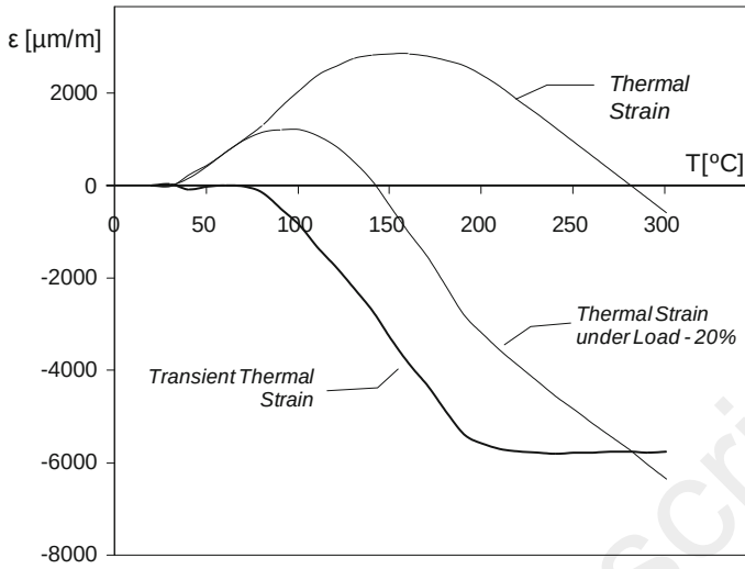
Fig. 5.55 Thermal strain, thermal strain under load and transient thermal strain for HPC cement paste (Hager 2004)
