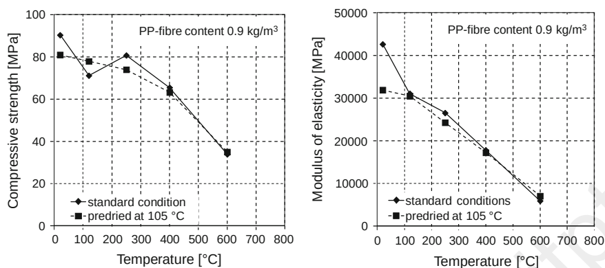
Fig. 5.12 Compressive strength (left) and modulus of elasticity (right) of high strength concrete with PP fibres for different preconditioning according to Hager (2004, c)
