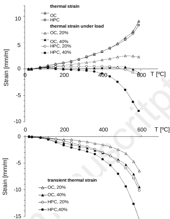
Fig. 5.44 Thermal strains, thermal strains under load and transient thermal strains for HPC and OC [results from Hager (2004), Hager and Pimienta (2005a, b)]
