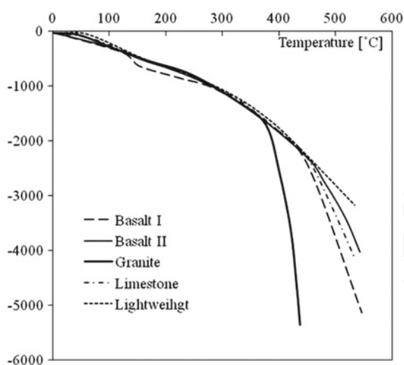
Fig. 5.47 Transient thermal strains (LITS in Khoury's nomenclature) of five concretes with different type of aggregates, measured during first heating ( 1^\circ\text{C}/\text{min} ) (Khoury 2006)
