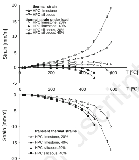
Fig. 5.45 Thermal strains, thermal strains under load and transient thermal strains for HPC with limestone aggregate and HPC with silico-calcareous aggregate [results from Hager (2004) and Hager and Pimienta (2005a)]
