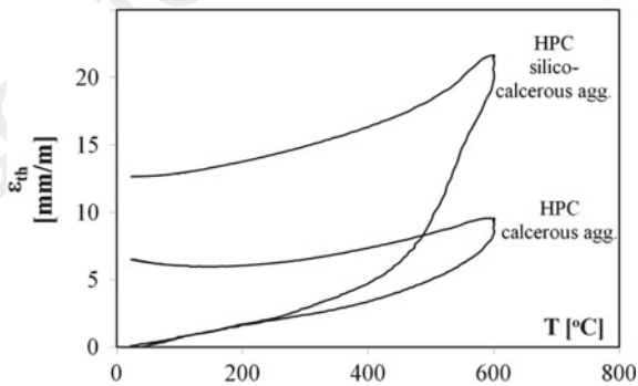
Fig. 5.40 Thermal strains of two HPCs containing silico-calcareous and calcareous aggregates. Samples heated to 600 °C and cooled down to the room temperature
