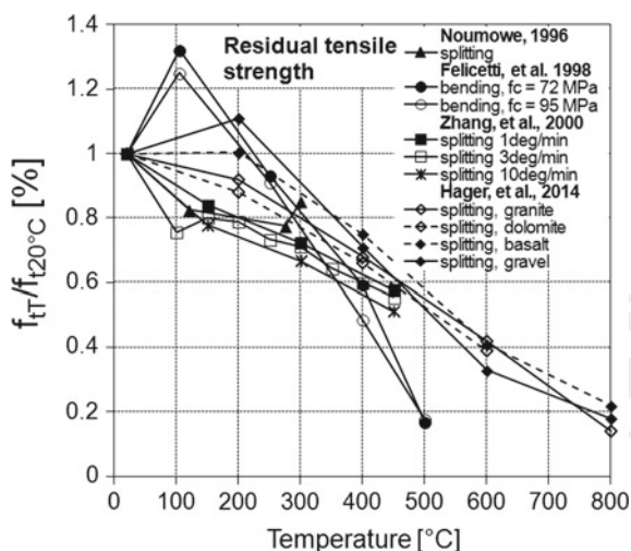
Fig. 5.60 Relative indirect tensile strength test results
