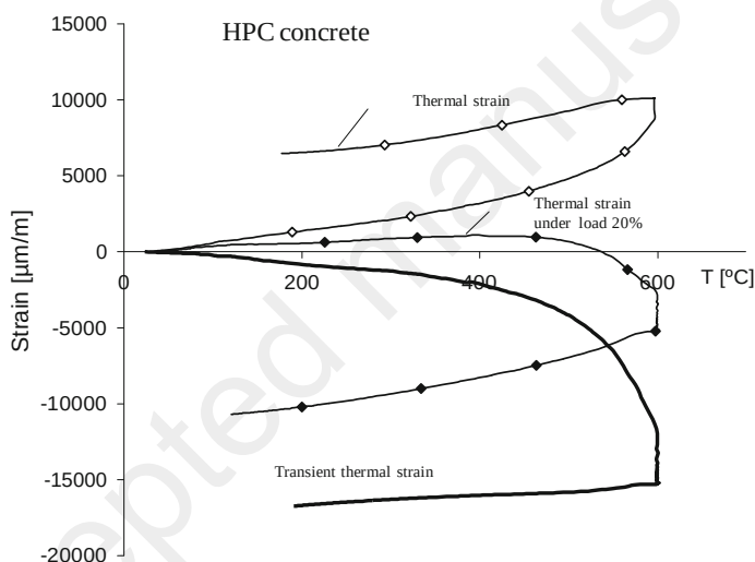
Fig. 5.51 Thermal strain, thermal strain under load and transient thermal strains of HPC sample during heating and cooling phase (Hager 2004)
