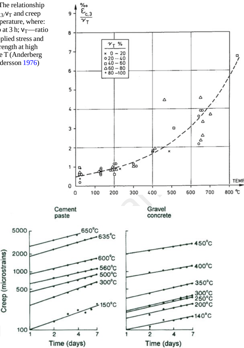
Fig. 5.32 Drying creep of high performance cement paste and gravel concrete (Khoury et al. 1986)
