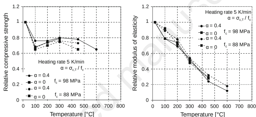
Fig. 5.16 Relative compressive strength (left) and relative modulus of elasticity (right) of two HPC with different load levels during heating according to Phan and Carino (2001)
