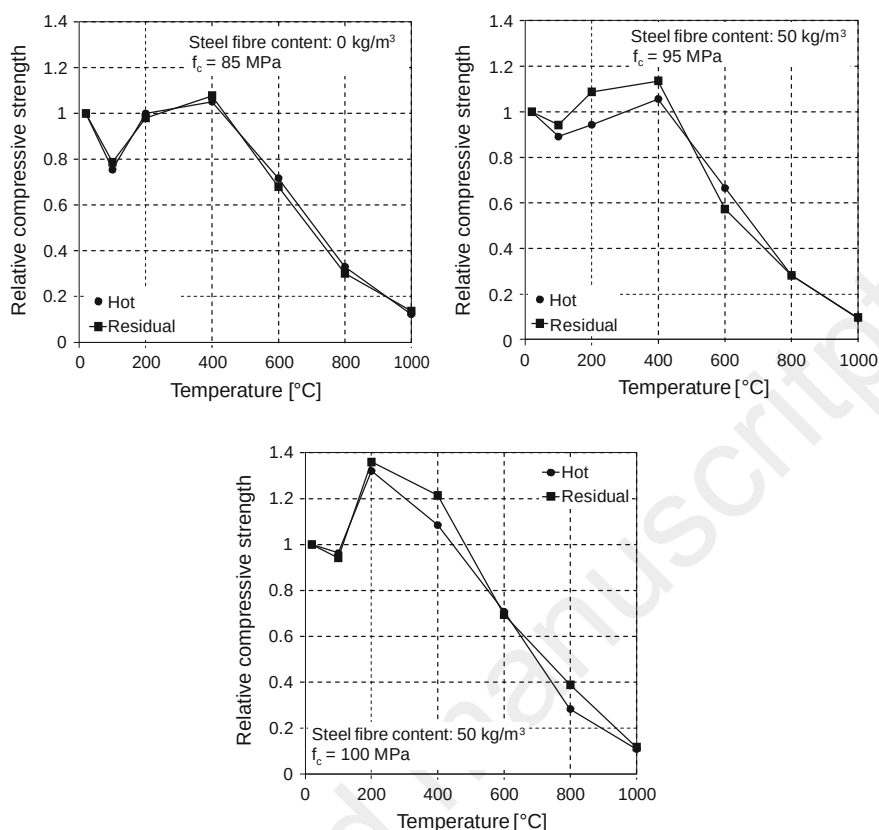
Fig. 5.21 Comparison of the “hot” and “residual” relative compressive strength of HPC with different amounts of steel fibres according to Horvath et al. (2004)
