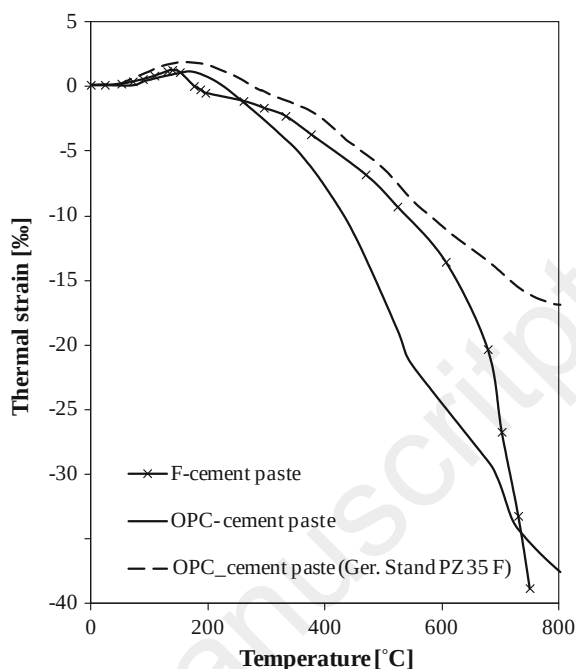
Fig. 5.38 Thermal strains of Portland cement pastes (OPC) and cement paste with blast furnace slag (F) (Jumppanen et al. 1986)
