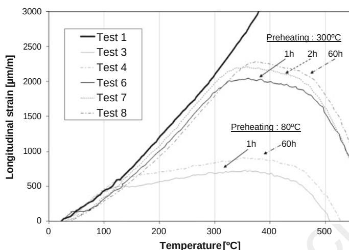
Fig. 5.54 Thermal strain and thermal strain under load of HPC samples with different states of dehydration. Influence of the pre-heating duration (Mindeguia 2009; Mindeguia et al. 2013)
