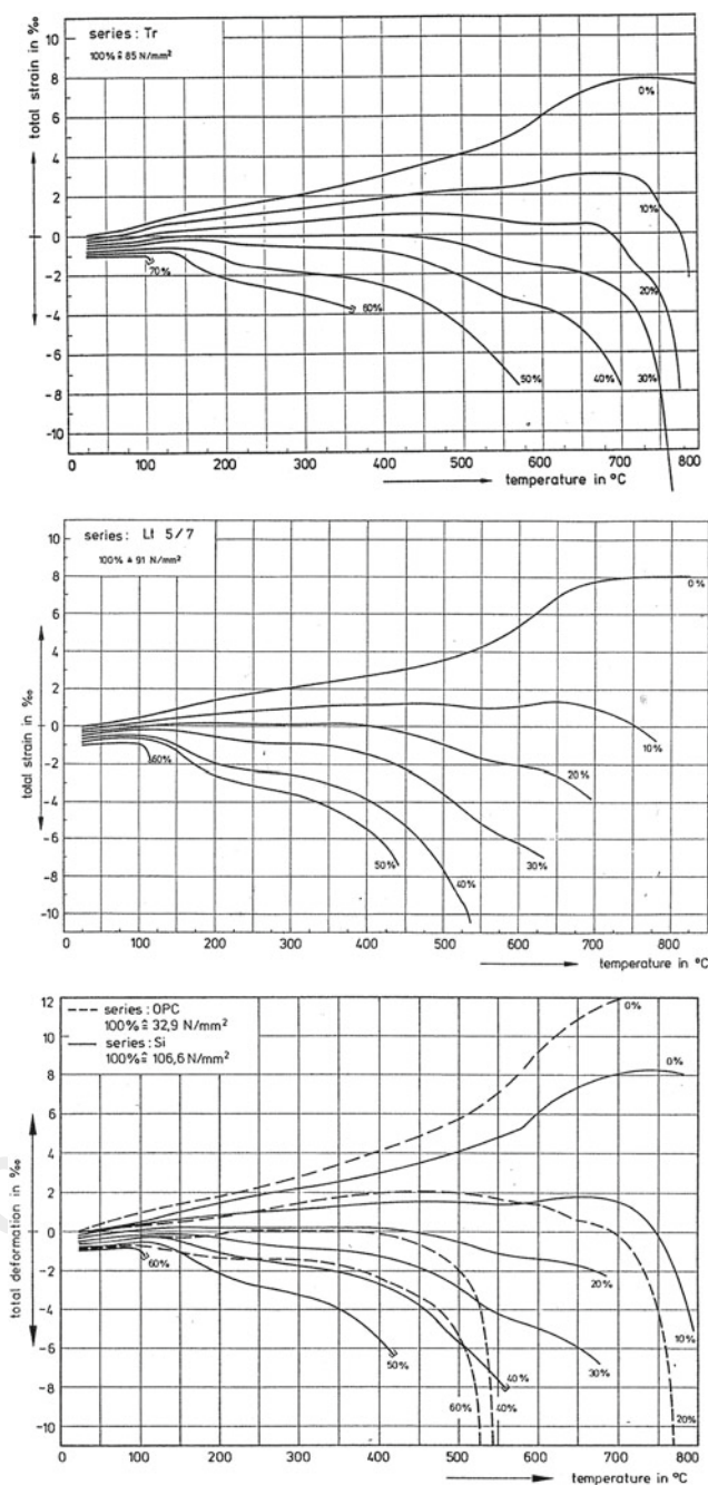
Fig. 5.48 Thermal strains and thermal strains under load of concretes made with different cement paste compositions (Diederichs et al. 1989). Fly ash (Lt), blast furnace slag (Tr), silica fume (Si), compared with ordinary Portland cement concrete
