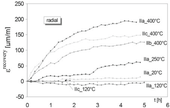
Fig. 5.34 Recovery of creep strains in radial direction (Mindeguia 2009)
