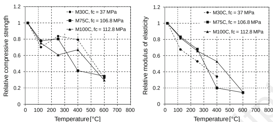
Fig. 5.3 Relative compressive strength (left) and modulus of elasticity (right) of normal and high strength concrete according to Pimienta and Hager (2002)
