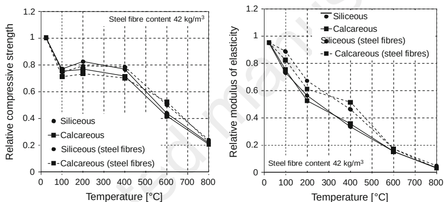
Fig. 5.11 Relative compressive strength and modulus of elasticity of HPC with and without steel fibres and different types of aggregates according to Cheng et al. (2004)
