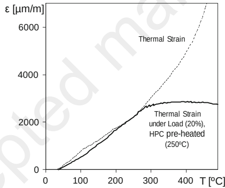
Fig. 5.53 Thermal strain and thermal strain under load of HPC in a sample pre-heated up to 250 °C, transient thermal strain is re-activated when T > 250 °C (Hager 2004)
