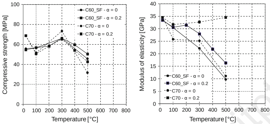
Fig. 5.17 Compressive strength (left) and modulus of elasticity (right) of two HPC with two different load levels during heating according to Khoury (1999)
