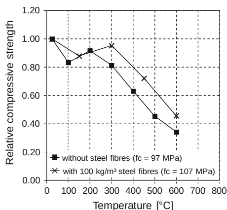
Fig. 5.10 Compressive strength of HPC with and without steel fibres according to Huisman et al. (2007)
