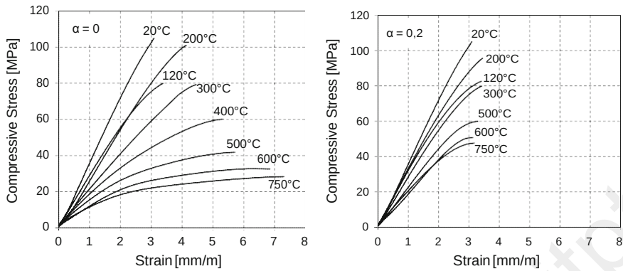
Fig. 5.1 Stress-strain curves of high strength concrete obtained in stress-rate-controlled tests (Huisman 2010)
