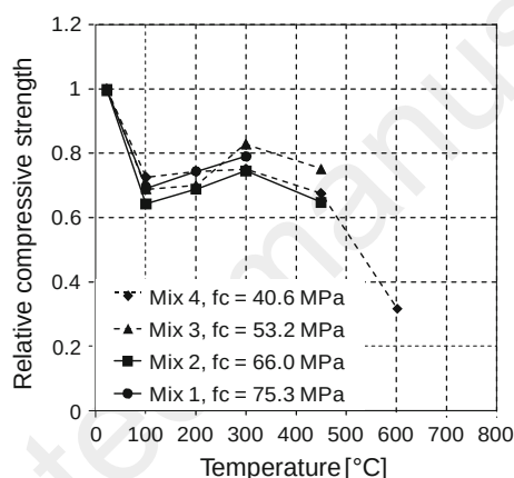
Fig. 5.4 Relative compressive strength of different concretes according to Phan and Carino (2001)
