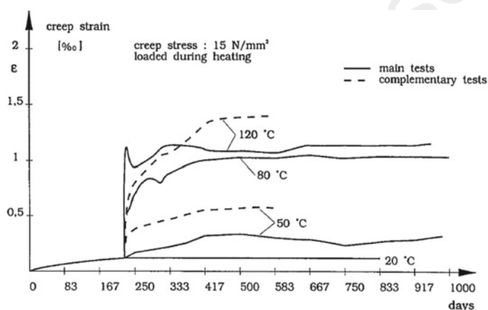
Fig. 5.25 Drying creep of HP basalt concrete, non-sealed samples (concrete tested at age of 3.5 years, and 90 days—complementary test) (Schneider 1982)
