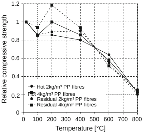
Fig. 5.22 Comparison of the “hot” and “residual” relative compressive strength of HPC with different amounts of PP-fibres according to Horvath et al. (2004)
