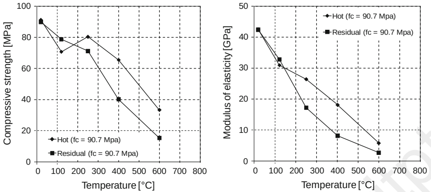
Fig. 5.19 Comparison of the “hot” and “residual” compressive strength (left) and modulus of elasticity (right) of high strength concrete according to Hager and Pimienta (2004a, b)
