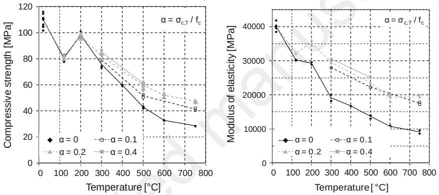
Fig. 5.14 Compressive strength (left) and modulus of elasticity (right) of one high strength concrete with different load levels during heating according to Huismann et al. (2009)
