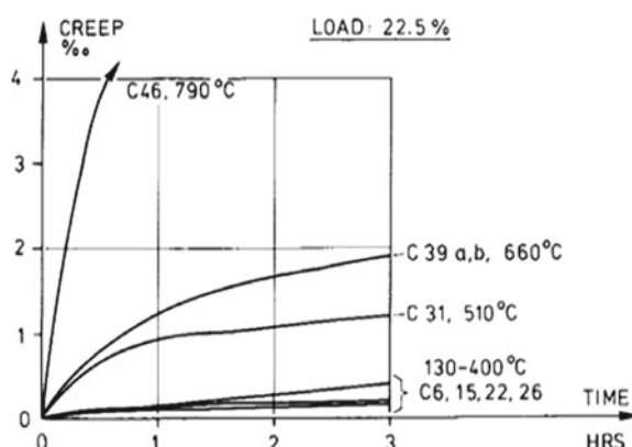
Fig. 5.29 Drying creep of concrete load level 22.5% (Anderberg and Thelandersson 1976)
