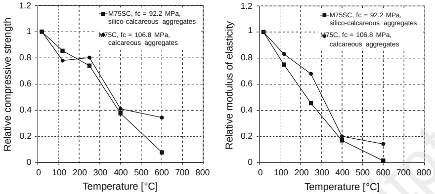
Fig. 5.5 Relative compressive strength (left) and relative modulus of elasticity (right) of two high strength concretes made with different aggregates according to Pimienta and Hager (2002) (“hot” tests)
