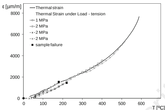
Fig. 5.56 Thermal strains and thermal strains under tensile load of HPC—now observable or absence of the transient thermal strains in tension (Mindeguia et al. 2013)
