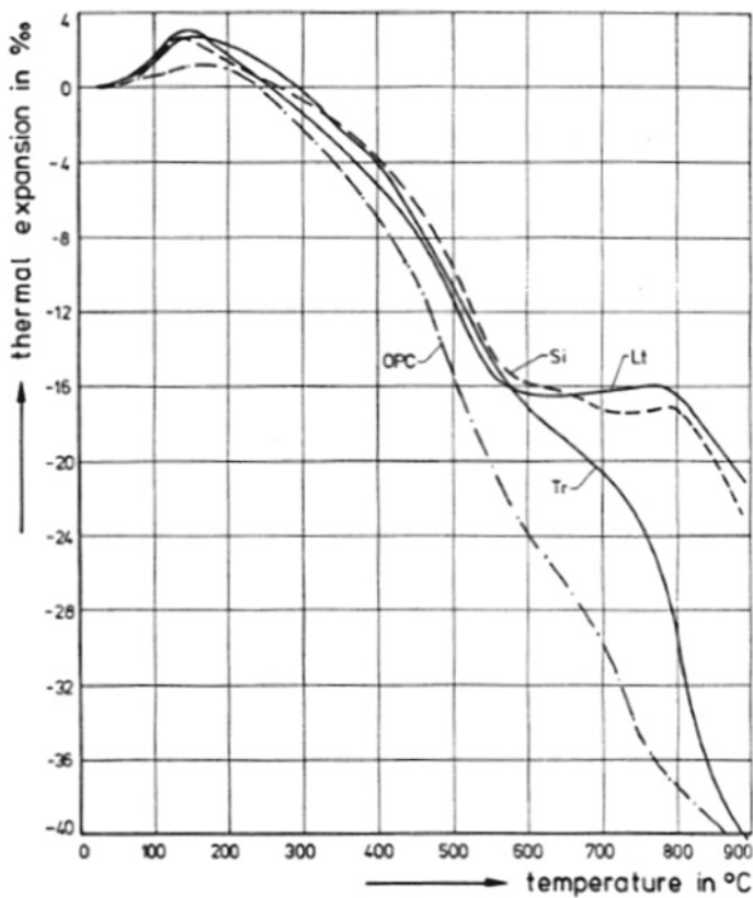
Fig. 5.39 Thermal strains of cement pastes (Diederichs et al. 1989). Silica fume (Si), fly ash (Lt), Portland cement (OPC) and blast furnace slag (Tr) cement pastes (Diederichs et al. 1989)
