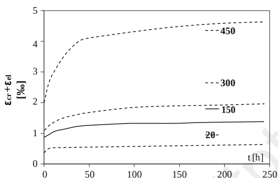
Fig. 5.28 Drying creep behaviour of concrete with quartz aggregates at 20, 150, 300 and 450 °C and load level of 0.3 by Schneider (1982)
