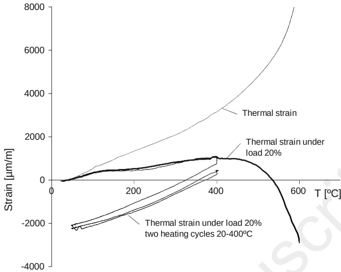
Fig. 5.52 Thermal strain under load curves of HPC sample after two cycles of heating at 400 °C (Hager 2004)
