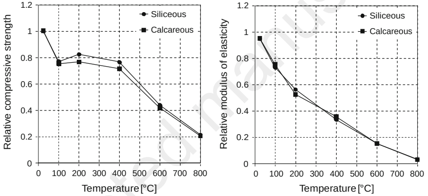
Fig. 5.6 Residual relative compressive strength (left) and relative modulus of elasticity (right) of two high strength concretes with aggregates according to Cheng et al. (2004) (residual tests)
