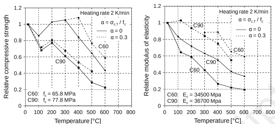
Fig. 5.15 Relative compressive strength (left) and relative modulus of elasticity (right) of two high strength concretes with two different load levels during heating according to Diederichs et al. (2009)
