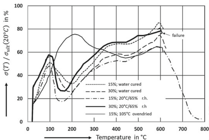
Fig. 5.58 Restrain forces of concretes made with Finnish aggregates and F-cement containing blast furnace slag (F) (Jumppanen et al. 1986)
