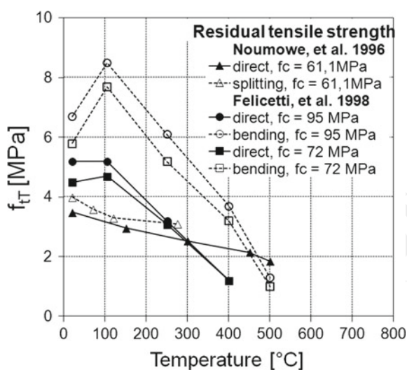
Fig. 5.61 The results of tensile strength obtained with different test methods
