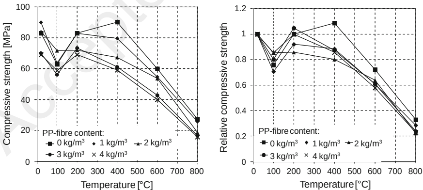
Fig. 5.8 Compressive strength (left) and relative compressive strength (right) of HPC made with different amounts of PP-fibres according to Horvath et al. (2004)
