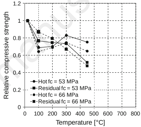
Fig. 5.19 Comparison of the “hot” and “residual” compressive strength (left) and modulus of elasticity (right) of high strength concrete according to Hager and Pimienta (2004a, b)
