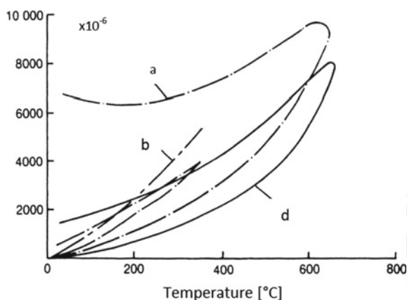
Fig. 5.36 Thermal strain of aggregates from Khoury et al. (1985a), a limestone b-gravel and d-basalt
