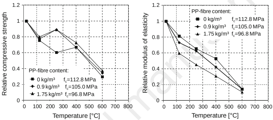
Fig. 5.7 Relative compressive strength (left) and modulus of elasticity (right) of high strength concrete made with different amounts of PP-fibres according to Hager and Pimienta (2004a)
