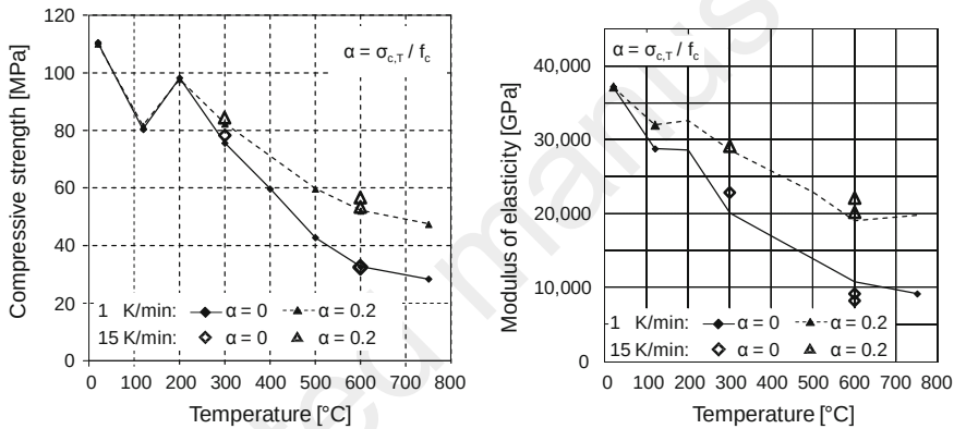
Fig. 5.18 Compressive strength (left) and modulus of elasticity (right) of HPC with two different load levels and heating rates according to Huismann (2010)
