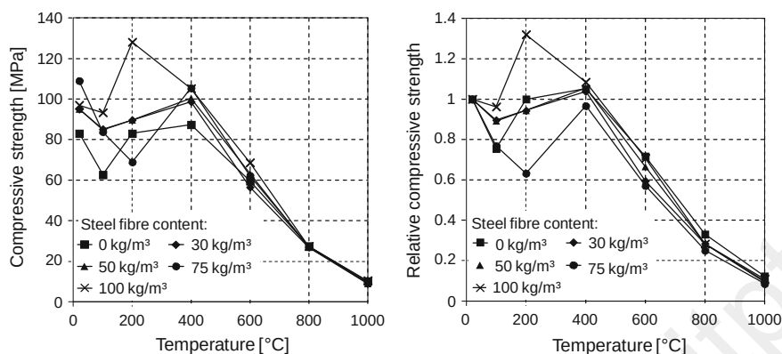
Fig. 5.9 Compressive strength (left) and relative compressive strength (right) of high strength concretes made with different amounts of steel fibres according to Horvath et al. (2004)
