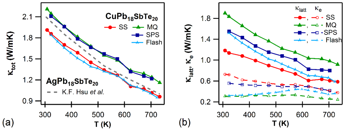
Figure 3. Thermal transport properties - (a) comparison of the total thermal conductivities, \kappa_{\text{tot}} of different \text{CuPb}_{18}\text{SbTe}_{20} samples vs \text{AgPb}_{18}\text{SbTe}_{20} (b) lattice, \kappa_{\text{latt}} and electronic, \kappa_e contributions to thermal transport
