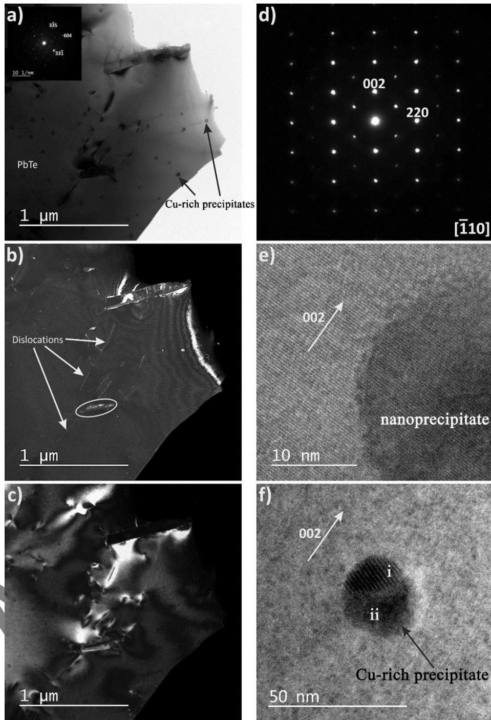
Figure 4. a) Bright Field (BF) image of \text{CuPb}_{18}\text{SbTe}_{20} (SS) thin sample. Inset shows the diffraction pattern, b) Dark Field (DF) image made with the \langle 3\bar{3}5 \rangle reflection depicting the dislocations, c) DF image made with the \langle 33\bar{1} \rangle reflection, d) Diffraction pattern along the [-110] zone axis, e) High magnification image showing the interface between the PbTe matrix and a Cu-rich nano-inclusion. f) High magnification image of the nanoprecipitate showing Moiré fringes in the upper part of the dark contrast domain (marked as i).
