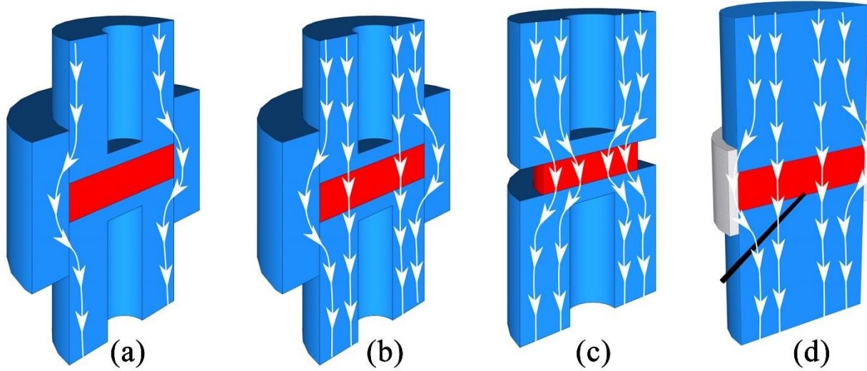
Figure 1. Flow of current in different sintering configurations - (a, b) In SPS set-up (with graphite punches and die) for high and low resistive samples, (c) Flash-SPS (graphite punches and no die), and (d) Hybrid Flash-SPS (graphite punches and a thin walled stainless steel die) configurations. Additional details pertaining to each configuration are presented in SI (Table S1).
