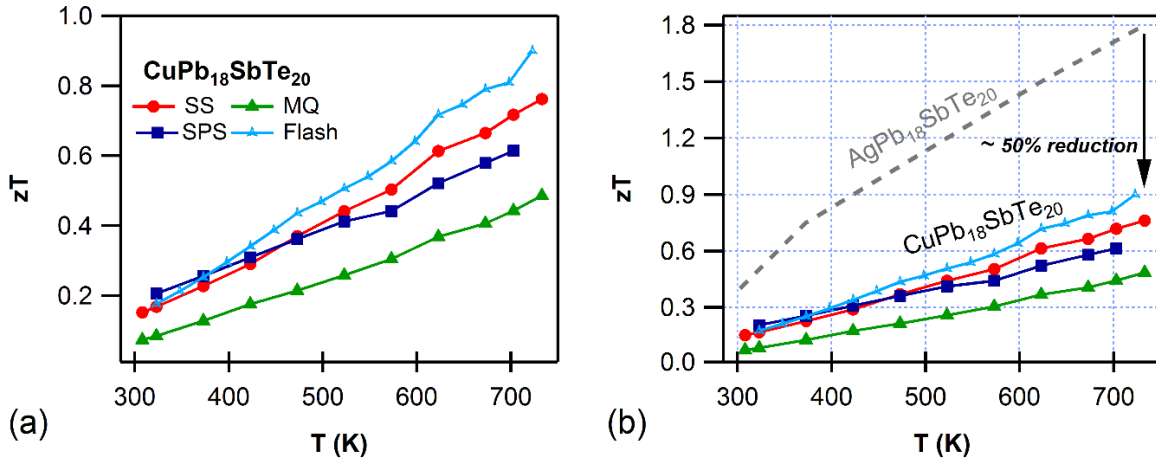
Figure 9. Temperature-dependent thermoelectric figure of merit, zT – (a) for \text{CuPb}_{18}\text{SbTe}_{20} samples that were prepared by different synthesis routes, (b) for different \text{CuPb}_{18}\text{SbTe}_{20} samples vs \text{AgPb}_{18}\text{SbTe}_{20} .
