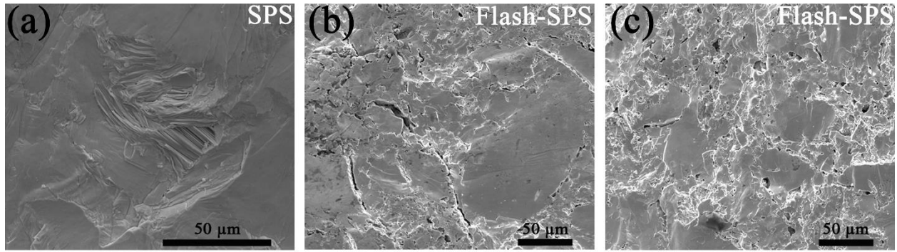
Figure 5. SEM images showing the microstructures at the fractured surface of (a) SPS sample with larger grains, (b, c) hybrid flash-SPS sample showing micro-porous voids and a mixture of larger and smaller grains.
