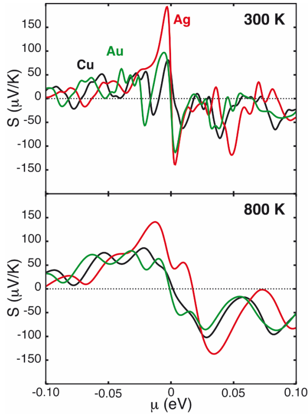
Figure 8. Thermopower as a function of the chemical potential ( \mu ) computed at 300 K (top) and 800 K (bottom) for MPb_{18}SbTe_{20} ( M = Cu, Ag, Au ) models.
