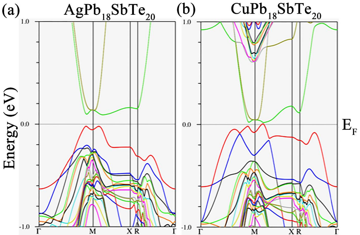
Figure 7. Electronic band structures computed for \text{MPb}_{18}\text{SbTe}_{20} ( M = \text{Cu}, \text{Ag} ). To compare the band structures, the same supercell was considered. Coordinates of high symmetry k -points: \Gamma = (0, 0, 0) , M = (\frac{1}{2}, \frac{1}{2}, 0) , X = (0, \frac{1}{2}, 0) , and R = (0, \frac{1}{2}, \frac{1}{2}) .
