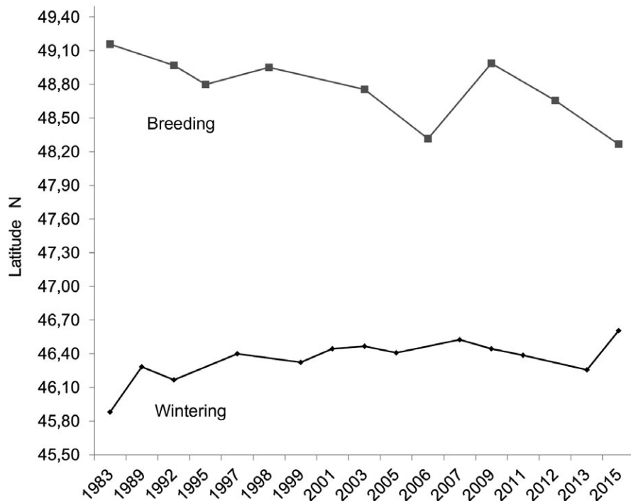
FIGURE 6 Change in the latitude of the weighted geographical centroid of wintering (a) and breeding (b) cormorants in France between 1983 and 2015
