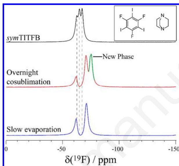
Figure 6. 19 F solid-state NMR ( v_{\text{MAS}} = 25 kHz) spectra of sample 4c obtained from slow evaporation (blue), overnight cosublimation (red), and the pure starting material (black). The new phase, assigned to structure 4c-iii , is shown in green. The dashed line serves as a guide.
