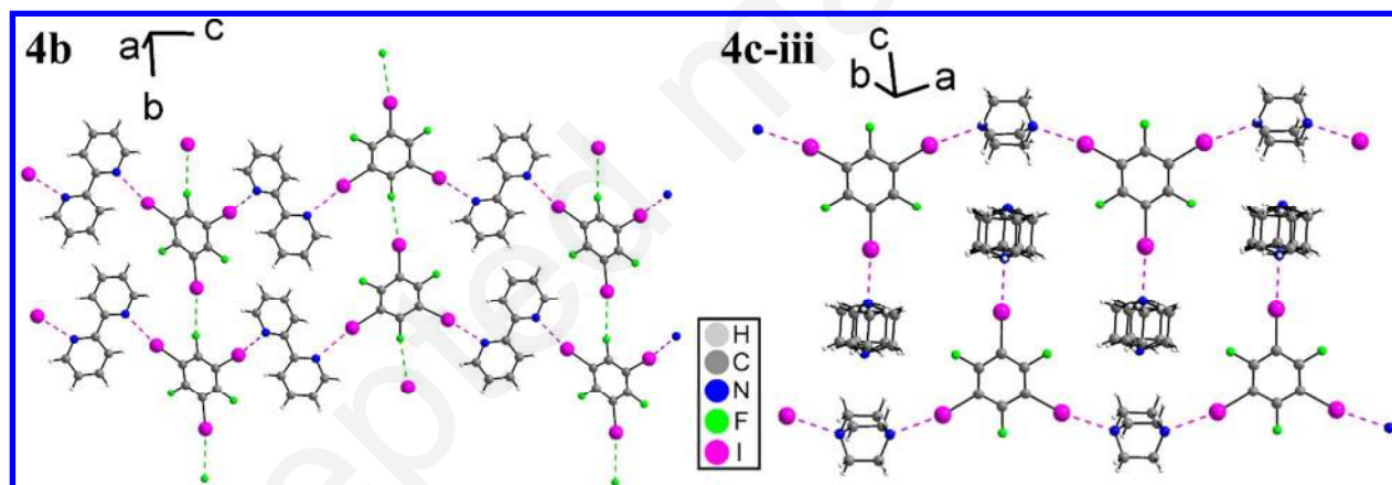
28 29 30 31 32 33 34 35 36 37 38 39 40 41 42 43 Figure 5. Crystal structures of 4b (left) and 4c-iii (right), obtained by cosublimation.
