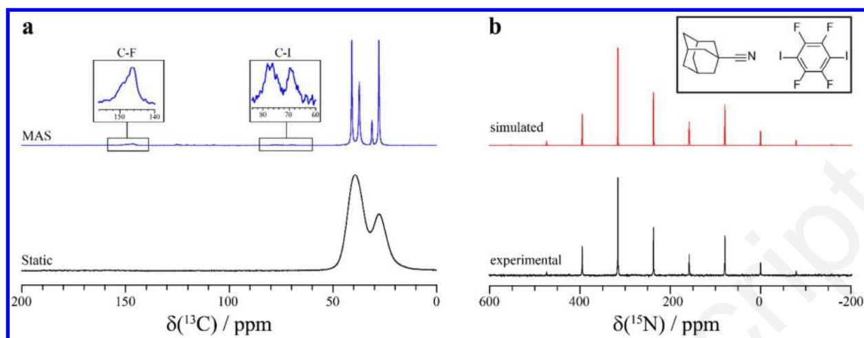
Figure 4. ^{13}\text{C} and ^{15}\text{N} (right) solid-state NMR spectra of compound 3d . (a) Experimental ^{13}\text{C} SSNMR spectra acquired under static (bottom left, black) and MAS conditions (upper, blue). Magnified views of the C-F and C-I resonances are shown in the insets. (b) Experimental ^{15}\text{N} SSNMR spectrum acquired at a 4 kHz MAS frequency (bottom, black), and the WSOLIDS 95 simulated spectrum (upper, red).
