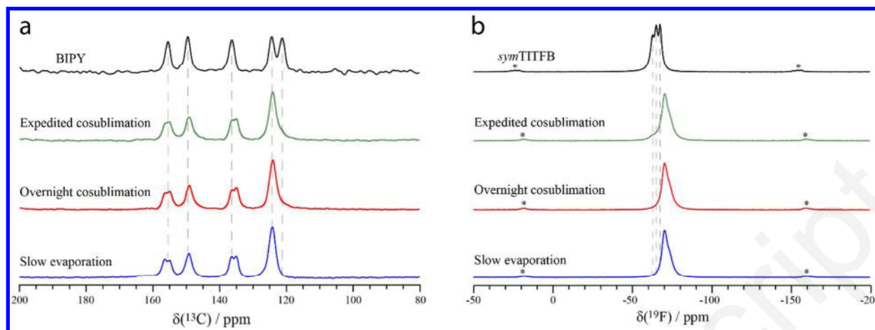
Figure 7. ^{13}\text{C} CP/MAS (a) and ^{19}\text{F} (b) MAS solid-state NMR spectra of compound 4b obtained from slow evaporation (blue), overnight cosublimation (red), expedited cosublimation (green), and their corresponding starting materials (black). The dashed lines serve as a guide to discern the starting material from the cocrystals. The asterisks denote spinning sidebands.
