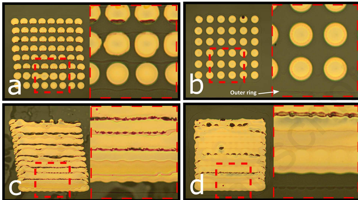
Figure 7: Optical pictures of square shaped patterns (approximately 1 \times 1 \text{ mm} ) printed at fixed UV ozone exposure time equals 10 minutes and varying:
