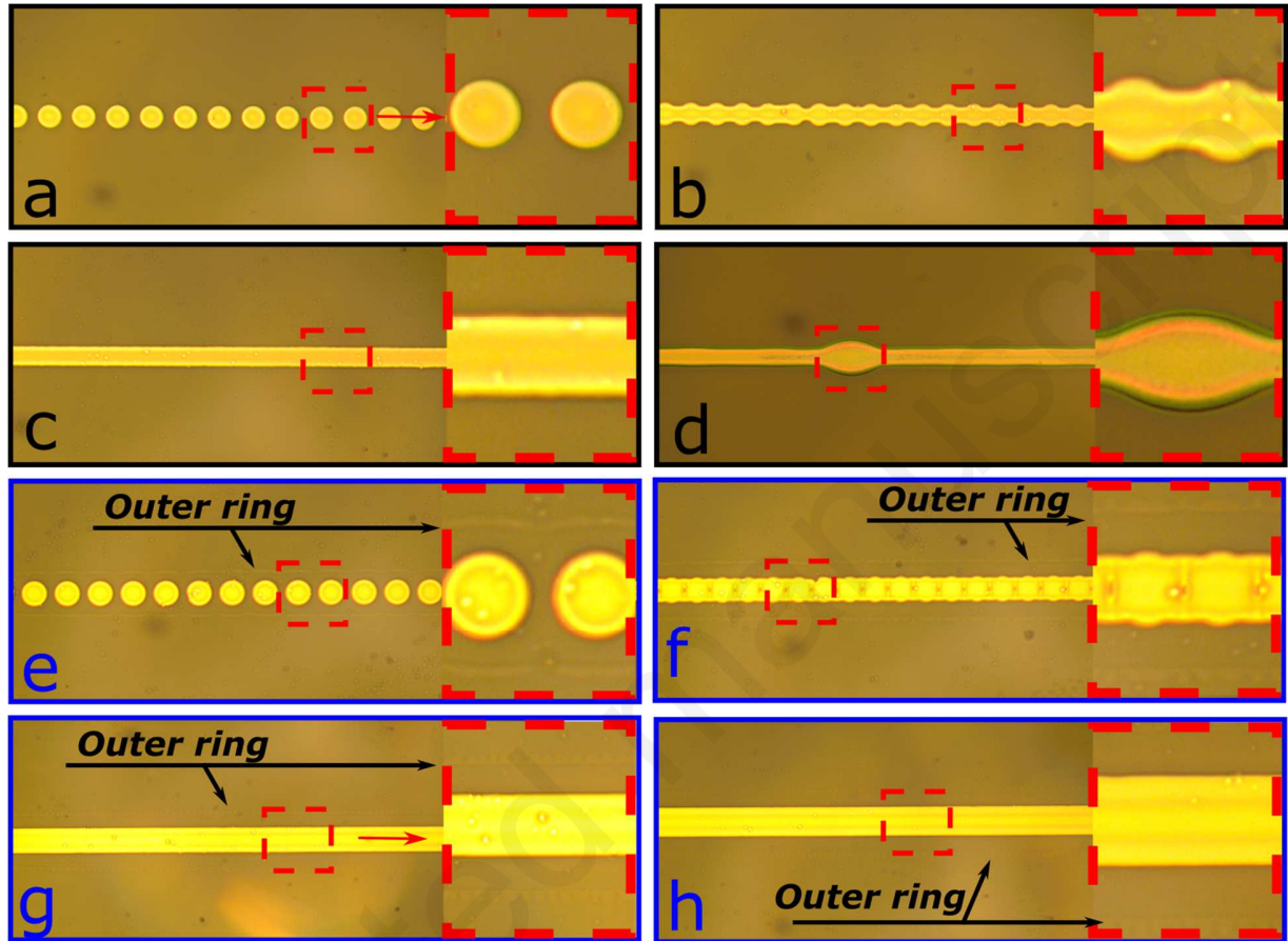
Figure 4: Lines formation mechanism as function of drop spacing and UV ozone exposure time. Jetting frequency equals 1 kHz. Hatched marks show zoom on lines. UV ozone time equals 2 minutes and drop spacing equals: a) 80 \mu m leading to isolated droplets, b) 60 \mu m leading to scalloped line, c) 40 \mu m leading to well defined lines, d) 25 \mu m leading to bulged line. UV ozone times equals 10 minutes and drop spacing equals: e) 200 \mu m leading to isolated droplets, f) 130 \mu m leading to scalloped lines, g) 70 \mu m leading to well defined line, h) 60 \mu m leading to well defined line.
