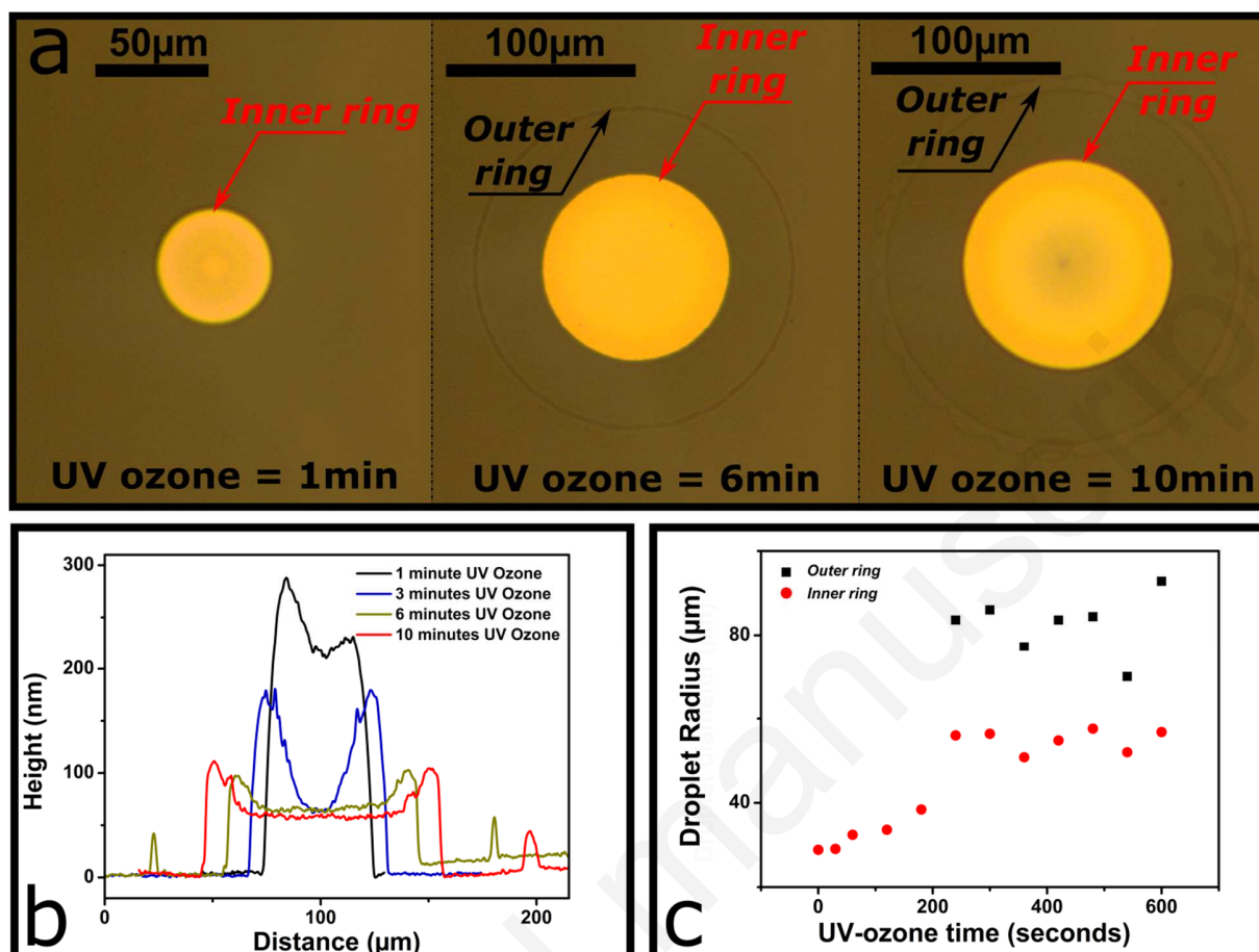
Figure 1: Morphological evolution of dried droplet as function of UV ozone effect. a) top view optical pictures of dried droplet as function of UV ozone time. UV ozone exposure time equals 1, 6 and 10 minutes (from left to right); b) Two dimensional profiles extracted along the diameter of a dried droplet as function of UV Ozone exposure time. UV ozone exposure time equals: 1, 3, 6 and 10 minutes; c) inner droplet diameter and outer droplet diameter as function of UV ozone exposure time.
