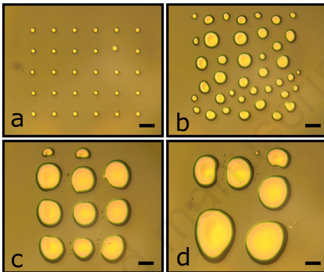
Figure S3: Square shaped patterns printed on polymeric surface (Su8 2000.5 MicroChem) without UV ozone treatment. Jetting frequency equals 1KHz and drop spacing equals: a) 100 \mu\text{m} leading to isolated droplets, b) 20 \mu\text{m} , c) 10 \mu\text{m} , d) 5 \mu\text{m} . In images b), c) and d), the printing parameters have been adjusted to overlap adjacent droplet leading to the coalescence of droplets and the formation of a stable pattern.
