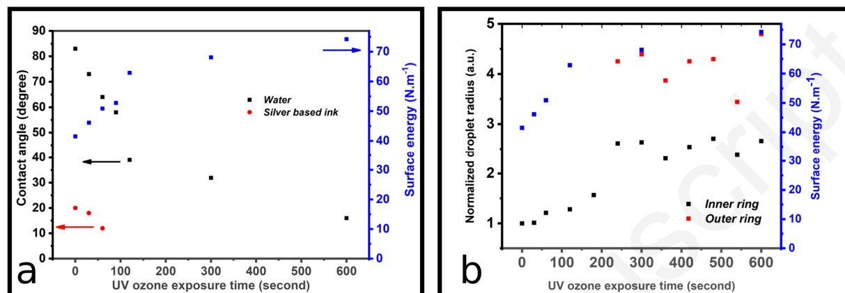
Figure S1: Spreading and wetting behavior of the droplets a) Water contact angle and silver based ink contact angle (left axis) as function of UV ozone exposure time . Note that, after 60 seconds silver based ink wets the surface totally and contact angle could not be measured. Surface free energy as function of UV ozone exposure time is plotted on right axis. Values confirm that the more the Su8 surface is exposed to UV ozone treatment, the more the surface becomes hydrophilic. b) Normalized droplet radii (inner and outer rings) and surface energy as function of UV ozone exposure time. The normalized radius show that the inner ring is about 2.5 times larger after 600s of exposure to UV ozone. The outer ring radius remains relatively consistent from its appearance (after 240s) to 600s exposure time.
