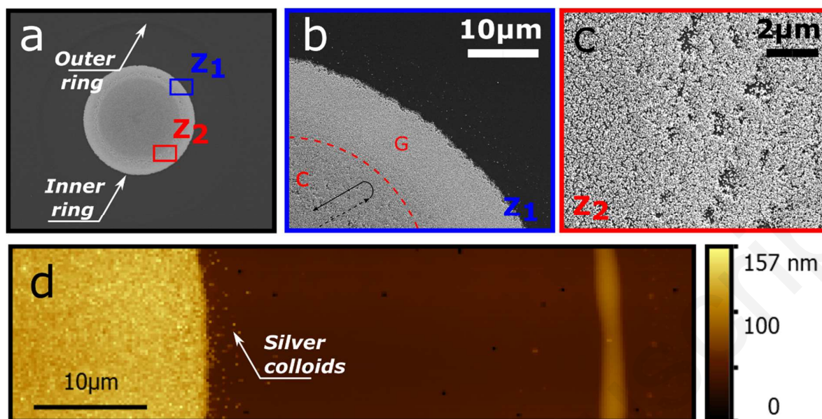
Figure S2: SEM pictures showing: a) dried droplet, b) A zoom Z1 showing the border between cap and foot; cap is divided in two regions named C and G. foot is the darkest region of the image; Black arrows shows internal flow in the C region during drying. c) A zoom Z2 showing inhomogeneity of dried nanoparticles in C region. d) AFM scan showing: colloid rich region (yellow region on left side of image) and polymer rich region (right side of the image). AFM image shows the only few amount of silver colloids can be found at the border of colloid and polymer rich region.
