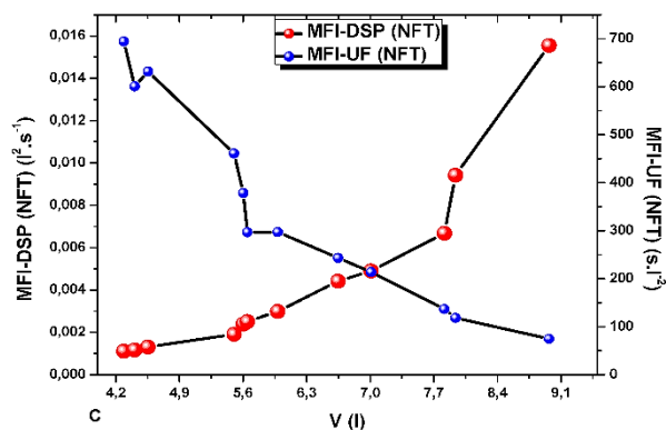
Figure 7: MFI – DSP evaluation according to the permeate volume, (A) in UFT, (B) in UFF and (C) in NFT, in polyethersulfone membrane of surface water filtration. ( T = 25^{\circ}\text{C} ; R_m = 8.140 \times 10^{13} \text{ m}^{-1} ; \Delta P_m = 2 \times 10^5 \text{ Pa} ; U_{if} = 0.111 \text{ m.s}^{-1} ; J_0 = 3.5 \cdot 10^{-5} \text{ m.s}^{-1} ; k_p = 1.92 \times 10^{-10} \text{ m/s.Pa} ; Q = 0.5 \text{ L/min} ).
