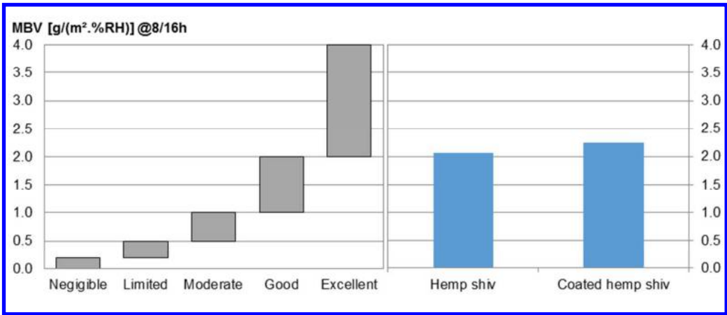
Figure 12: Practical moisture buffer value classes and moisture buffer values of hemp shiv and coated hemp shiv
