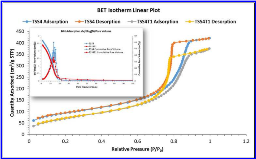
Figure 3: N 2 adsorption-desorption isotherms of silica (TSS4) and functionalised silica (TSS4T1). The insert is the BJH pore distribution of both samples.
