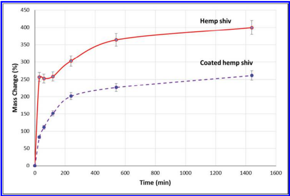
Figure 11. Dependence of water absorption on time for hemp shiv and coated hemp shiv
