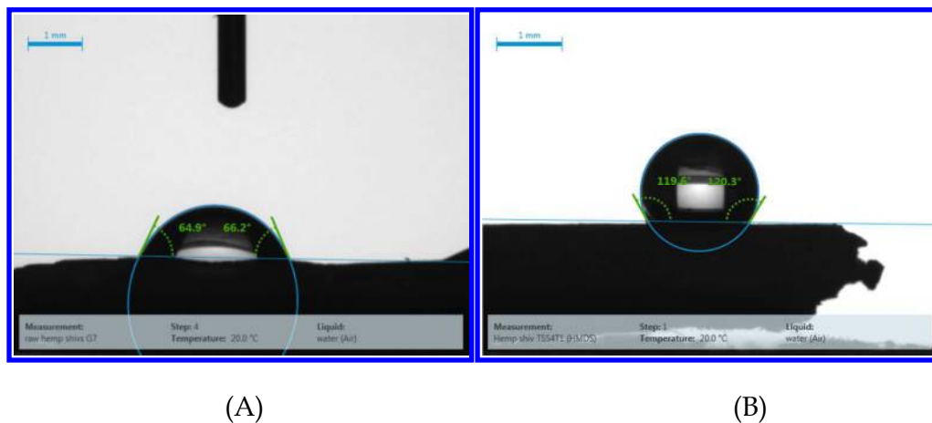
Figure 10: Water contact angle of raw hemp shiv (A) and coated hemp shiv (B). Note: Image is one of five measurements
