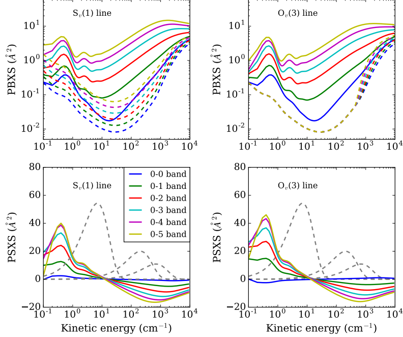
Figure 1: Comparison of pressure broadening and shifting cross sections between S_v(1) and O_v(3) lines in various vibrational bands at different kinetic energies (solid lines). The index v denotes the final vibrational quantum number. The inelastic contributions to the PBXS are presented in the upper panels (dashed lines). The Maxwell-Boltzmann distributions at 10, 296 and 1000 K are represented as dashed gray lines in the lower panels.
