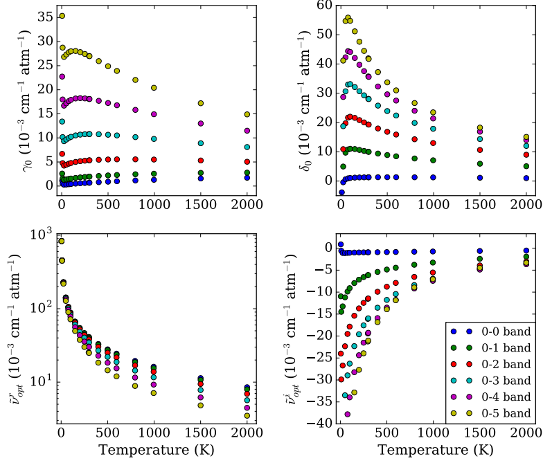
Figure 7: Pressure broadening, \gamma_0 , and pressure shift, \delta_0 , coefficients, real and imaginary parts of the Dicke parameter, \tilde{\nu}_{opt}^i , for the S_v(1) lines as a function of temperature.
