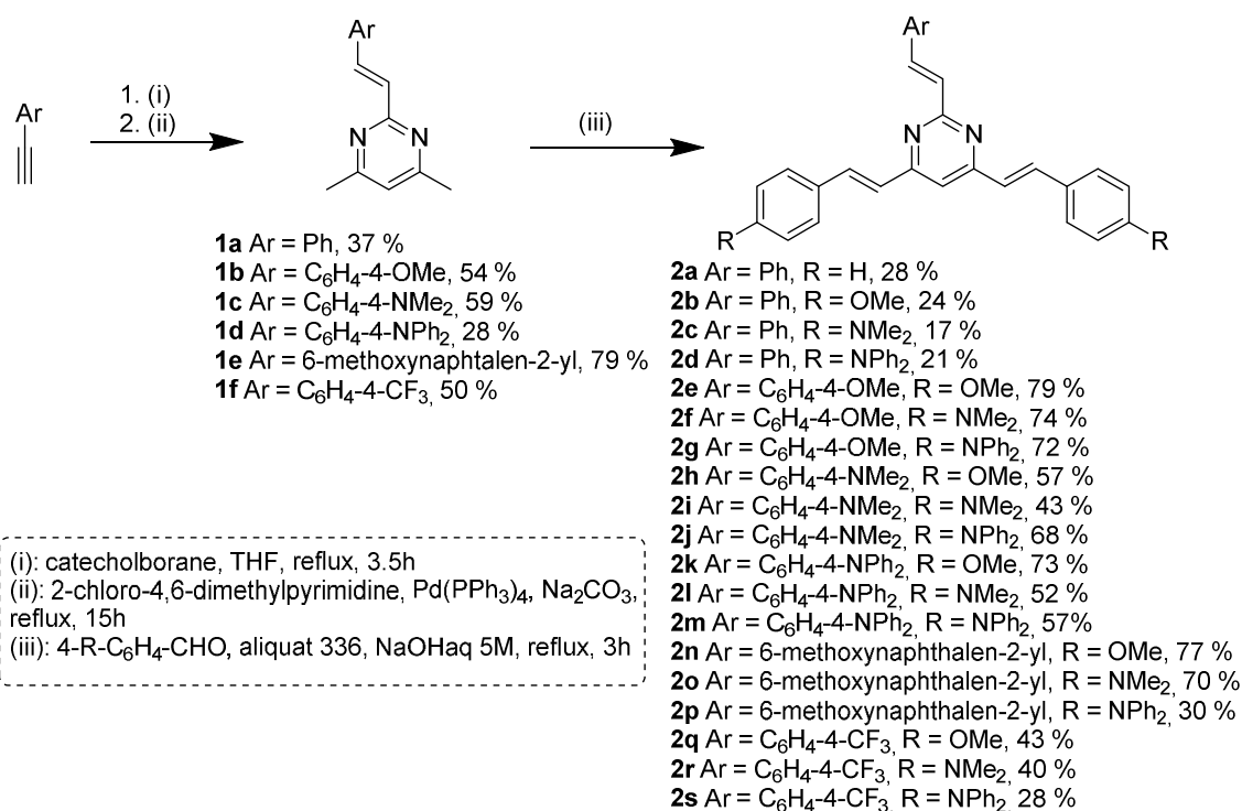
Scheme 1: Synthesis of compounds 2 .
