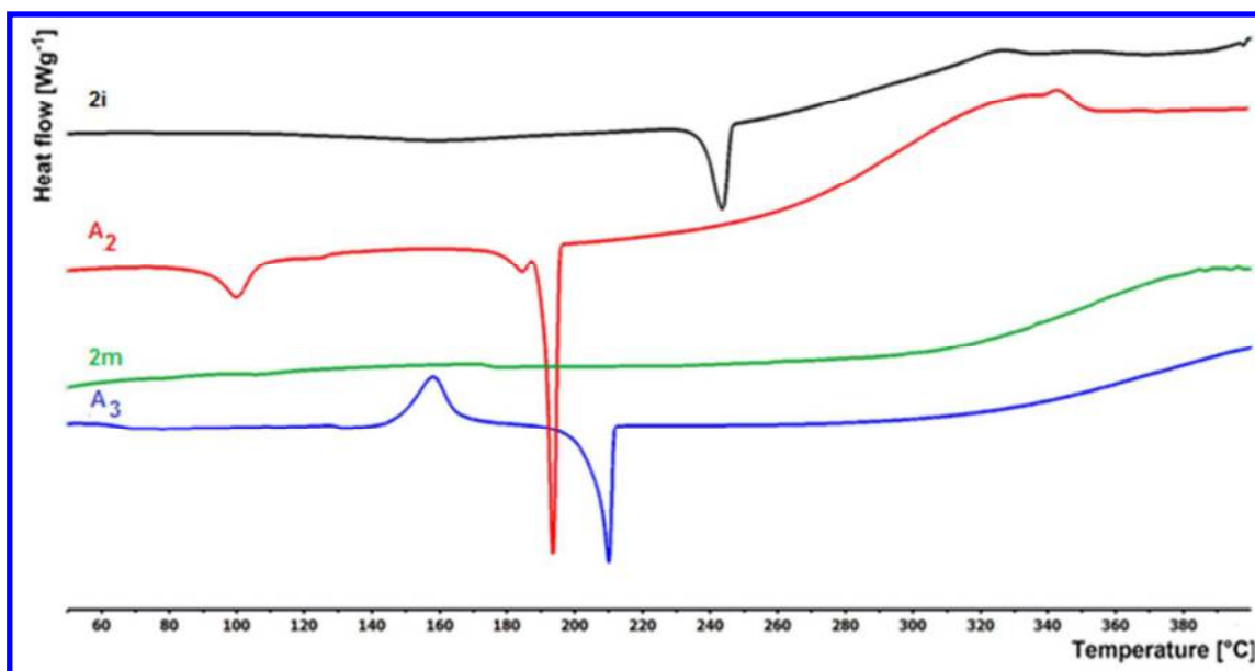
Figure 2: Representative DSC thermographs of compounds 2i , 2m , A 2 and A 3 obtained with a scanning rate of 3°C/min in the range 50-400°C
