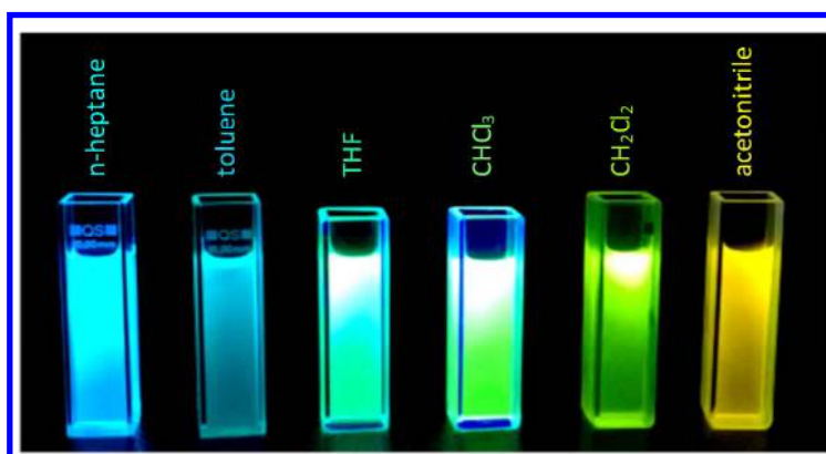
Figure 5: Fluorescence color changes experienced by 2k in various solvents. Picture was taken in the dark upon irradiation with a hand-held UV lamp ( \lambda_{\text{em}} = 366 \text{ nm} ).
