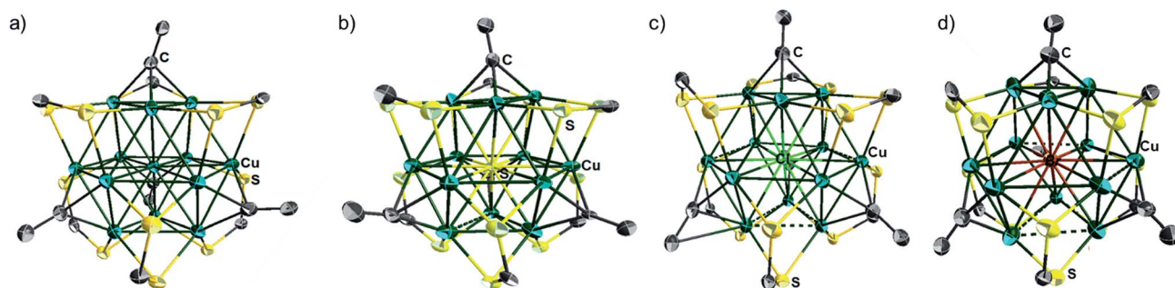
Fig. 3 Single crystal structures of the cluster cation 1a (a), cluster 2a (b), cluster cations of 3e (c) and 4e (d) with 30% thermal probability ellipsoids. All n\text{Bu} , \text{C}(\text{O})\text{OMe} ( 1a , 2a ) and phenyl ( 3e , 4e ) moieties are omitted for clarity.
