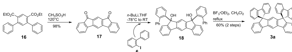
Scheme 5. Synthesis of 3a -Route A
