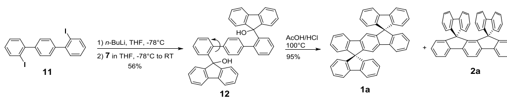
Scheme 3. Synthesis of 1a and 2a -Route B
