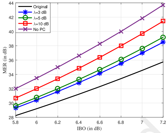
Fig. 5. MER with QCQP for DVB-T2 with 64 QAM in 2K mode with Rapp model HPA, p = 10 .
