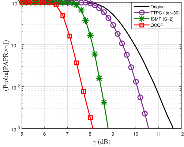
Fig. 11. CCDF of PAPR with QCQP, ICMP and TTPC for DVBS-T2 with 64QAM in 2K mode.
