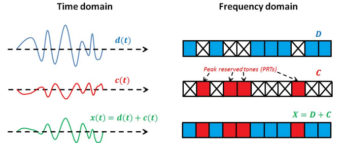
Fig. 2. Typical illustration of a TR scheme.
