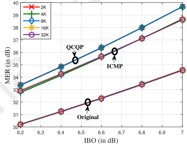
Fig. 13. MER for original signal along with QCQP and ICMP for DVBS-T2 with 64QAM for various FFT sizes with Rapp model HPA, p = 10 .
