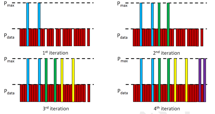
Fig. 10. Iterative power allocation of the PRTs with GICMP in the frequency domain.
