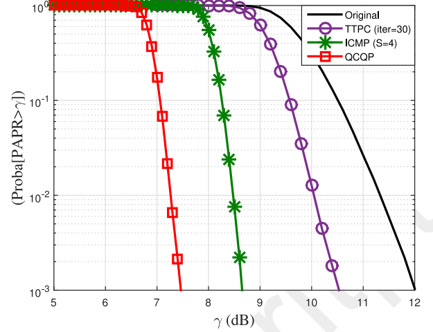
Fig. 12. CCDF of PAPR with QCQP, ICMP and TTPC for DVBS-T2 with 64QAM in 8K mode.
