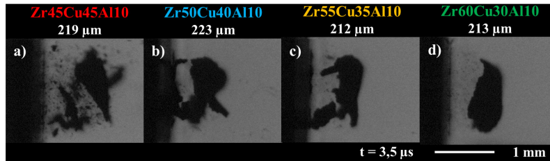
FIGURE 2. Transverse shadowgraphy of Zr_{45}Cu_{45}Al_{10} , Zr_{50}Cu_{40}Al_{10} , Zr_{55}Cu_{35}Al_{10} , and Zr_{60}Cu_{30}Al_{10} samples at 3.5 \mu s after a 1.3 PW.cm^{-2} intensity laser-shot. Every shot was in identical laser conditions (energy, duration, spot diameter and sample thickness).
