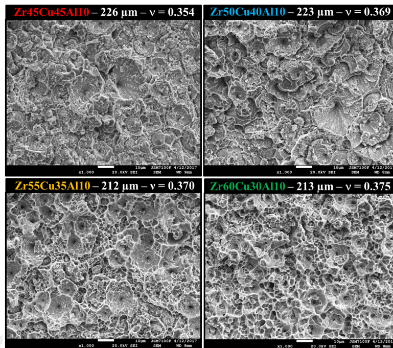
FIGURE 3. SEM magnification of spalled areas of Zr_{45}Cu_{45}Al_{10} , Zr_{50}Cu_{40}Al_{10} , Zr_{55}Cu_{35}Al_{10} , and Zr_{60}Cu_{30}Al_{10} samples recovered after 1.3 PW.cm^{-2} laser-shock. Corresponding Poisson's ratios (related to zirconium content) are indicated.
