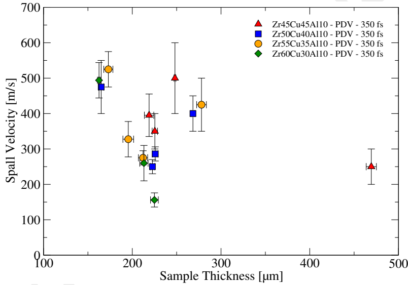
FIGURE 1. Spall velocity evolution versus sample thickness of Zr_xCu_{(90-x)}Al_{10} samples ( x = 45 red triangle, x = 50 blue square, x = 55 yellow circle, and x = 60 green diamond) subjected to 1.3 \text{ PW.cm}^{-2} intensity laser shock.
