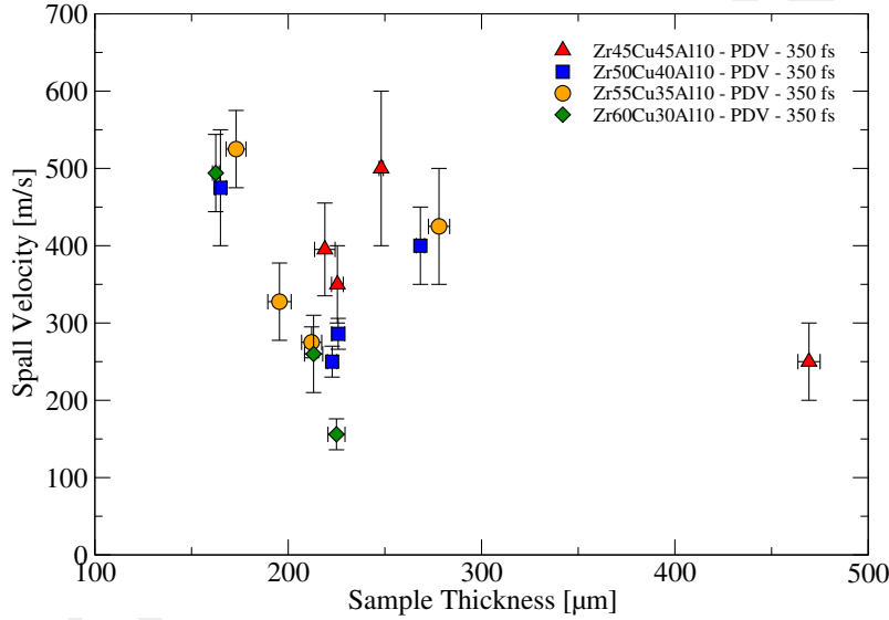
FIGURE 1. Spall velocity evolution versus sample thickness of \text{Zr}_x\text{Cu}_{(90-x)}\text{Al}_{10} samples ( x = 45 red triangle, x = 50 blue square, x = 55 yellow circle, and x = 60 green diamond) subjected to 1.3 \text{ PW.cm}^{-2} intensity laser shock.
