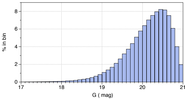
Fig. 20. Magnitude distribution for \sim 507\,000 Gaia sources that are not included in Gaia -CRF2, but are tentatively identified as quasars through a cross-match with the MILLIQUAS catalogue.
