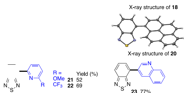
Scheme 1. Scope of Aryl Bromides in Palladium-Catalyzed Direct C4 Arylation of 2,1,3-Benzothiadiazole
