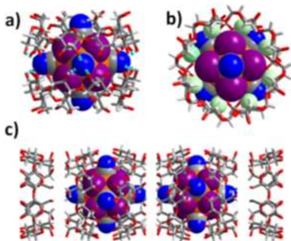
Figure 2. Mixed representations of the solid state structure of the supramolecular host-guest \{[\text{Re}_6\text{Q}_8(\text{CN})_6]-(\gamma\text{-CD})_2\}^{4+} complex with Q = Se or Te: a) side view showing the hydrogen bonding between the equatorial cyano groups and the hydroxyls of the primary faces of the CDs; b) top view highlighting close interactions between inner H-3 hydrogen (pale-green sphere) and four Q ligands (violet sphere) with \text{H}\cdots\text{Q} = 3.1\text{-}3.5 \text{ \AA} ; c) focus on the linear "bamboo-like" arrangement running along c axis.
