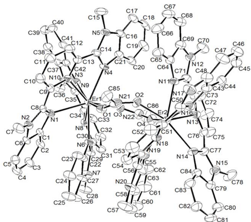
Figure S38 ORTEP molecular view with numbering scheme of the asymmetric unit for [(L4)_2Er((CH_3)NO_2)_2Er(L4)_2]^{6+} in the crystal structure of 10 . Thermal ellipsoids are represented at the 40% probability level and hydrogen atoms are omitted for clarity.
