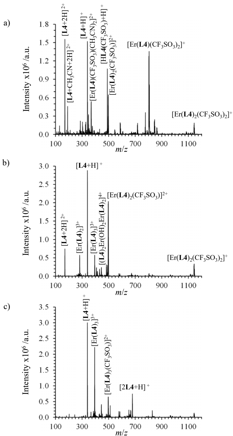
Figure S9 ESI-MS spectra recorded upon titration of L4 with Er(CF 3 SO 3 ) 3 (total ligand concentration: 2.0×10 -3 M in acetonitrile, 298 K) for stoichiometric ratios a) [Er] tot / [L4] tot = 1.00, b) [Er] tot / [L4] tot = 0.50 and c) [Er] tot / [L4] tot = 0.33.
