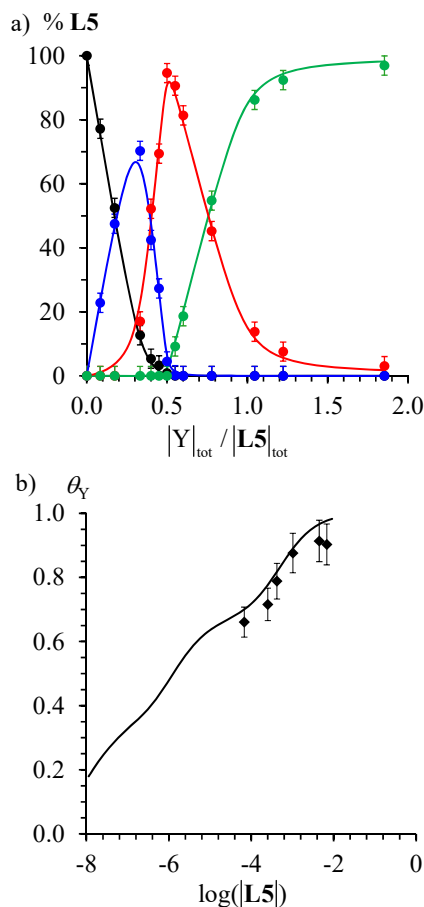
Figure 3. a) Macroscopic ligand speciations (dots) obtained by integration of ^1\text{H} NMR signals during the titration of \mathbf{L5} ( 1.6 \times 10^{-2} \text{ mol} \cdot \text{dm}^{-3} ) with \text{Y}(\text{CF}_3\text{SO}_3)_3 in \text{CD}_3\text{CN} at 298 K (black = \mathbf{L5} , blue = [\text{Y}(\mathbf{L5})_3]^{3+} , red = [\text{Y}(\mathbf{L5})_2]^{3+} and green = [\text{Y}(\mathbf{L5})]^{3+} ) and b) associated binding isotherm (Eq. (7); diamonds). The full traces correspond to the re-constructed a) distribution and b) binding isotherm computed using Equilibria (4)-(6) with \beta_{1,1}^{Y,\mathbf{L5}} = 8.0 , \beta_{1,2}^{Y,\mathbf{L5}} = 13.9 and \beta_{1,3}^{Y,\mathbf{L5}} = 17.2 .
