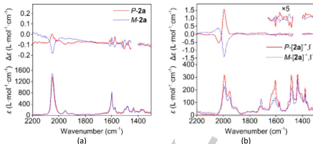
Figure 6. (a) VCD spectra (up) and IR spectra (down) for P -2a (red solid) and M -2a (blue dashed). (b) VCD spectra (up) and IR spectra (down) of P -[2a] + ,I - (red solid) and M -[2a] + ,I - (blue dashed). Noticeable different intensities in the IR spectra in P - and M -[2a] + ,I - may be due to concentration errors and incomplete oxidation upon I 2 addition. See Ref. [9] for the corresponding data for 2b/[2b] + ,I - .
