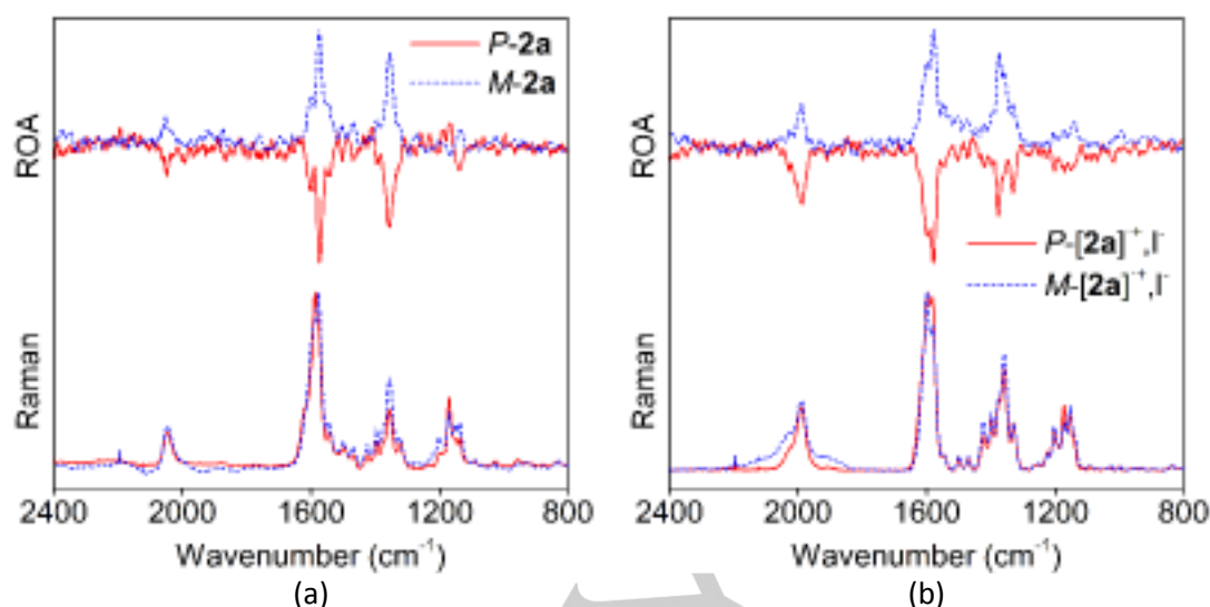
Figure 8. (a) ROA spectra (top) and Raman spectra (bottom) for P - 2a (red solid) and M - 2a (blue dashed). (b) ROA spectra (top) and Raman spectra (bottom) for P -[ 2a ] +,I- (red solid) and M -[ 2a ] +,I- (blue dashed). See Ref. [9] for the corresponding data for 2b /[ 2b ] ••2+ .
