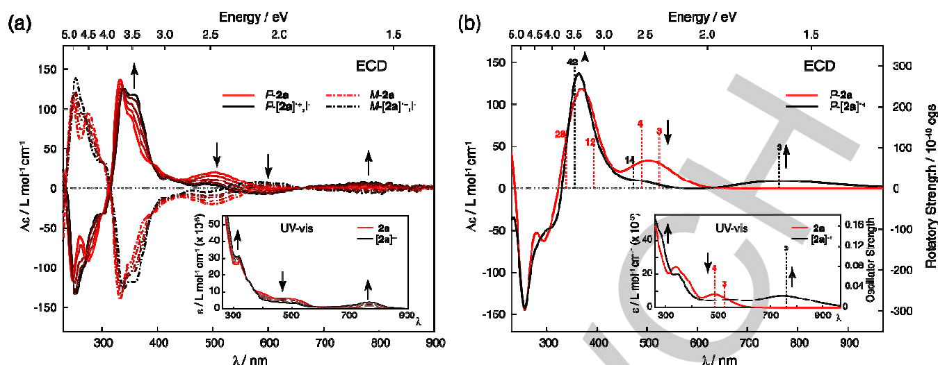
Figure 4. (a) Evolution of the ECD spectrum of 2a upon its oxidation with iodine. ECD spectra of P-2a (plain red), oxidized species P-[2a] •+ (plain black) and their corresponding enantiomers M-2a and M-[2a] •+ (dotted lines) in \text{CH}_2\text{Cl}_2 ( C\ 10^{-5}\ \text{M} ). Inset: Spectroelectrochemical oxidation studies of 2a with potentials from -0.2 to +0.4 V (vs. Ag pseudo-electrode) in \text{C}_2\text{H}_4\text{Cl}_2 , \text{NBu}_4\text{PF}_6 (0.2 M). [9] (b) Simulated (B3LYP/SV(P), Boltzmann-averaged for two conformers) ECD spectra of P-2a (red line) and P-[2a] •+ (black line). Inset: The corresponding UV-vis spectra. No spectral shift was applied. Calculated excitation energies and rotatory / oscillator strengths indicated as 'stick' spectra. Numbered excitations for the lowest-energy conformers for each species (respectively, 2a-I and [2a-II] •+ ) were analyzed in detail (see Table 1 and SI).
