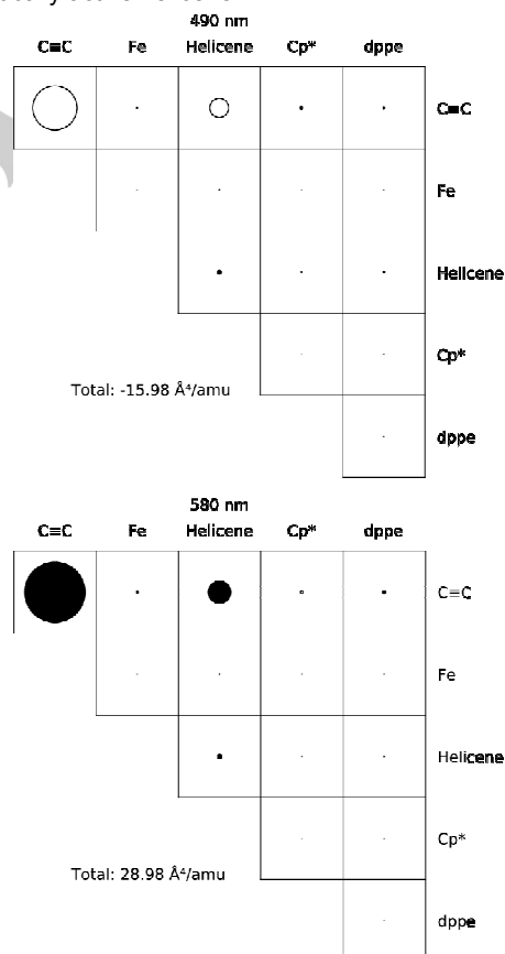
Figure 10. Intensity distribution of the alkynyl stretching mode over different parts of M-2a for 490 nm (top) and 580 nm (bottom) incident laser wavelength. We adopt the coupling-matrix representation introduced by Hug. [29]
