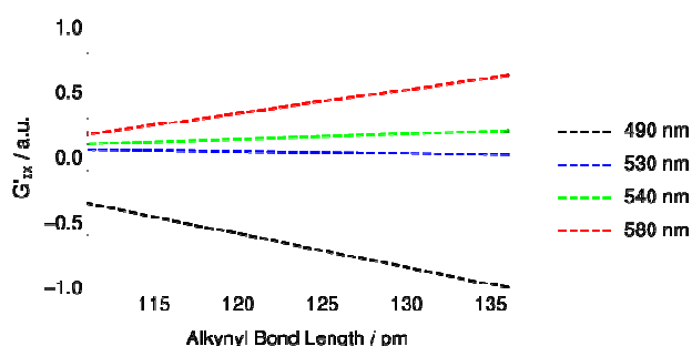
Figure 11. xx element of the electric dipole-magnetic dipole polarizability tensor G' , as a function of the alkynyl bond length for different wavelengths of the incident laser beam. Note that for each wavelength, G' has only been calculated for two bond lengths (111 pm and 136 pm); the dashed lines are not intended to imply a linear relationship but only to help visualizing the trend. Note also that the values of G'_{xx} were normalized to the absolute value of the largest element.
