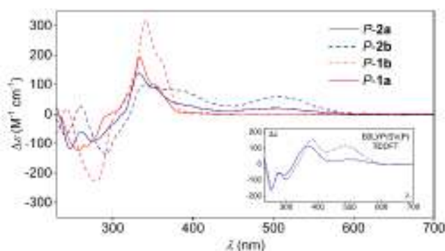
Figure 1. ECD spectra of P - 1a (plain red), P - 2a (plain blue), P - 1b (dashed red) and P - 2b (dashed blue) in \text{CH}_2\text{Cl}_2 ( 1 \cdot 10^{-5} \text{ M} ). [9] Inset: Simulated (B3LYP/SV(P)) spectra of P - 2a and P - 2b (see also SI).
