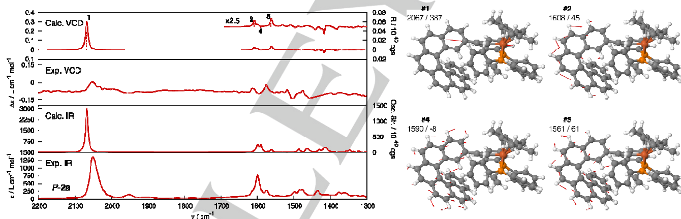
Figure 7. Left: Comparison of experimental and calculated (B3LYP/SV(P) gas-phase, frequencies scaled by 0.96, Boltzmann-averaged for two conformers) IR (down) and VCD (up) spectra of 2a. Numbered VCD vibrations correspond to those analyzed in detail for 2a-I. Right: Atomic displacement for the numbered normal modes in 2a-I. Numbers listed are the corresponding vibrational frequency (in cm -1 , scaled) / rotatory strength (10 -44 cgs) values. See also SI.
