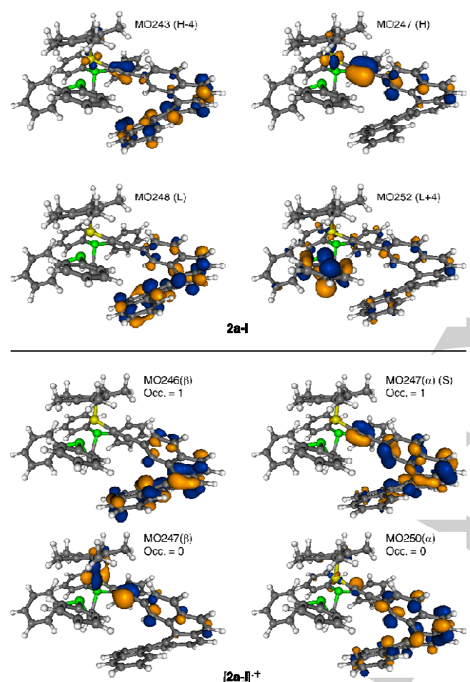
Figure 3. Isosurfaces ( \pm 0.04 au) of MOs involved in selected electronic excitations of 2a/[2a] •+ (conformer I). 'H' = HOMO, 'L' = LUMO, 'S' = SOMO. The corresponding MOs for 2b/[2b] •+2+ can be found in Ref. [9]. See also SI for a full set of MOs for both systems.
