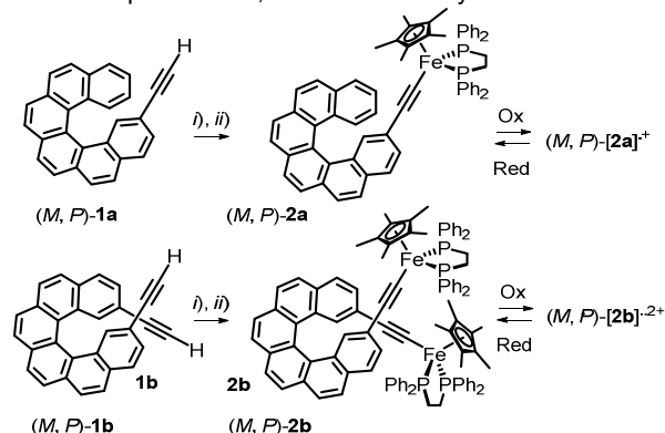
Scheme 1. Organometallic mono- and bis-iron-ethynyl-carbo[6]helicene derivatives 2a,b obtained from mono- and bis-ethynyl-carbo[6]helicenes 1a,b , and their redox-switching processes. i) \text{Fe}(\kappa^2\text{-dppe})(\eta^5\text{-C}_5\text{Me}_5)\text{Cl} , MeOH, THF, \text{NaPF}_6 ; ii) THF, t\text{BuOK} . [9]
