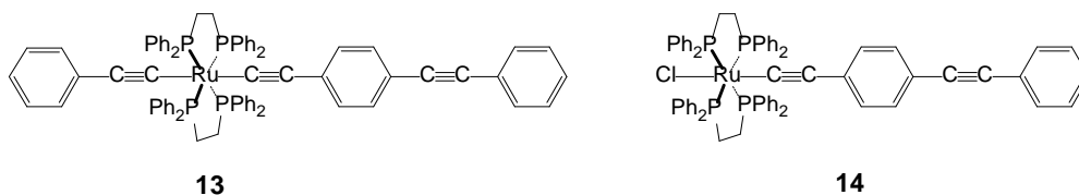
Chart 3. Related complexes previously assessed by femtosecond Z-scan. 17
