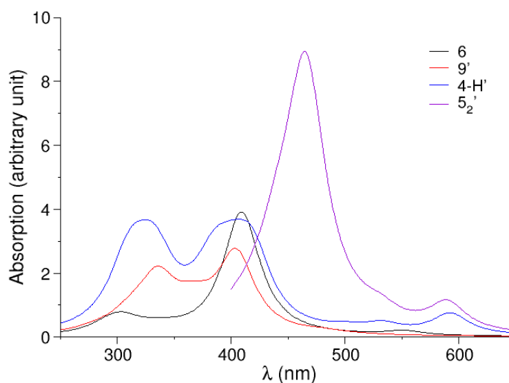
Figure 5. Calculated UV-vis absorption spectra of the compounds 4-H' , 5 2 ' , 6 , and 9' . Computations were carried out up to 400 nm for 5 2 ' due to computational limitations.
